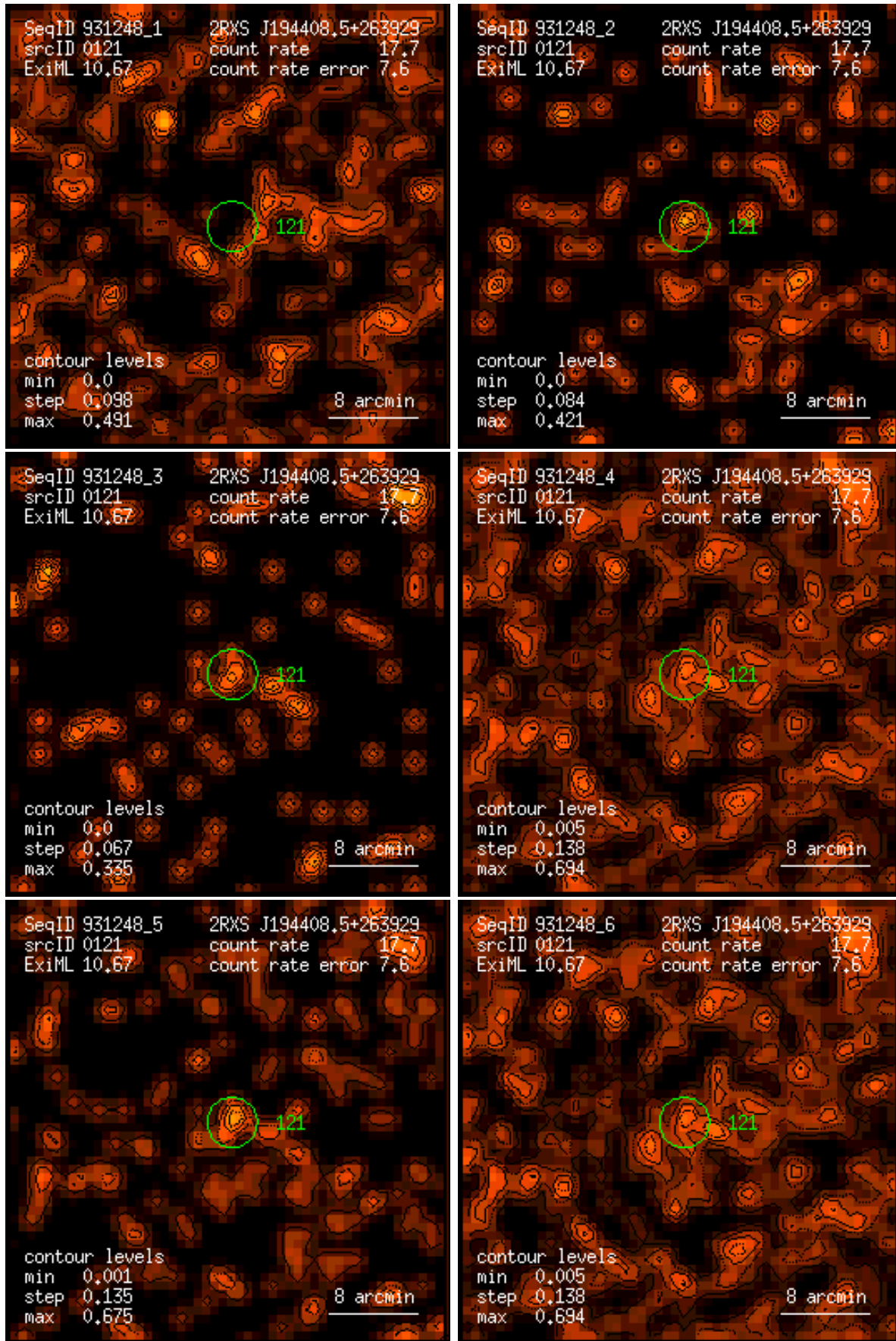
Figure 121: RASS 931248: detection 0121: band rate images, Gaussian filter: (1) PSPC channels 11 – 41, (2) 52 – 90, (3) 91 – 201, (4) 11 – 235, (5) 52 – 201, (6) 11 – 201. Broad band rates in counts/ks. Band rate contour levels in counts/ks/arcmin 2 .
