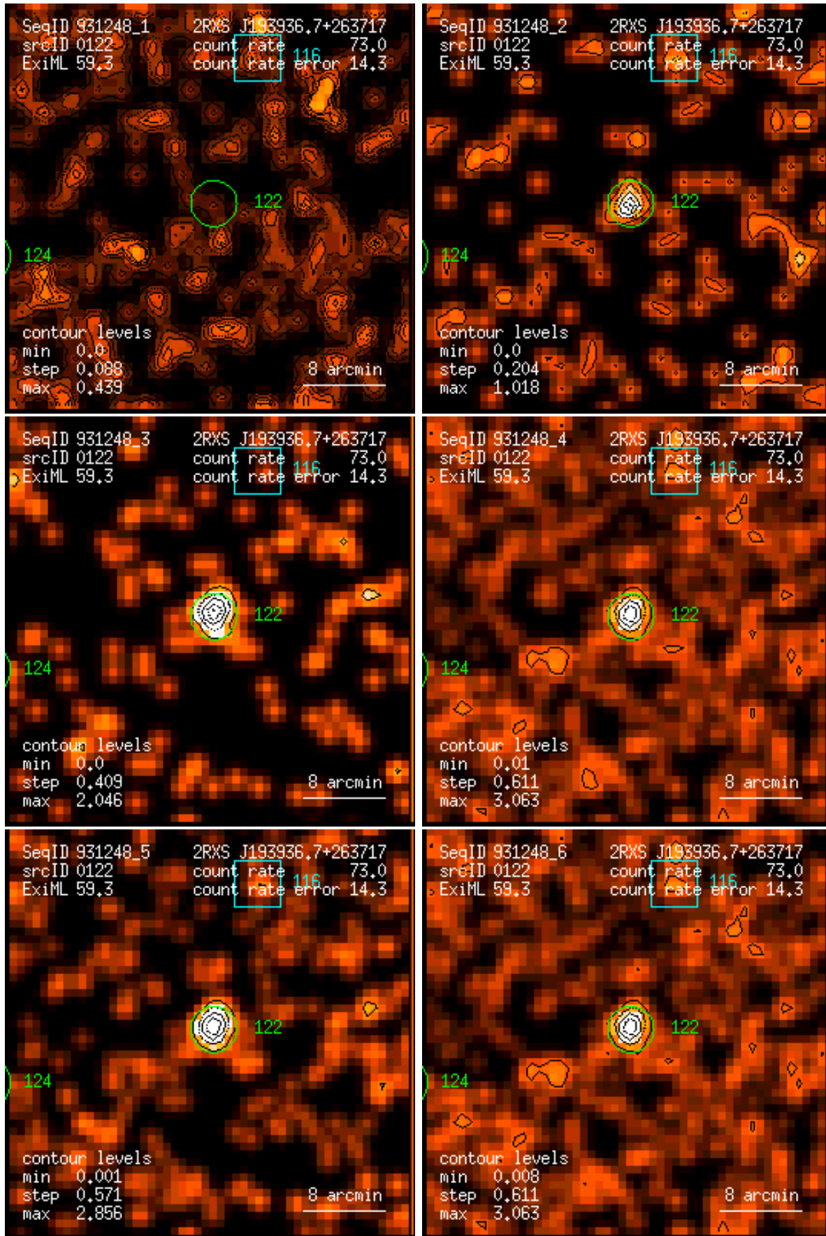
Figure 122: RASS 931248: detection 0122: band rate images, Gaussian filter: (1) PSPC channels 11 – 41, (2) 52 – 90, (3) 91 – 201, (4) 11 – 235, (5) 52 – 201, (6) 11 – 201. Broad band rates in counts/ks. Band rate contour levels in counts/ks/arcmin 2 .
