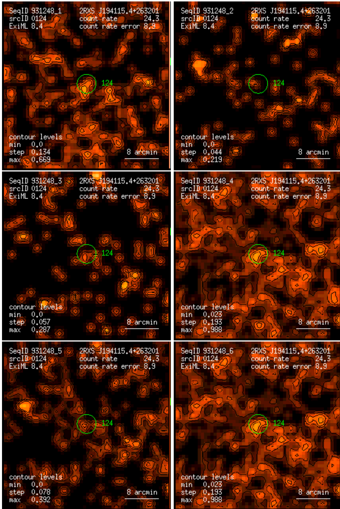
Figure 124: RASS 931248: detection 0124: band rate images, Gaussian filter: (1) PSPC channels 11 – 41, (2) 52 – 90, (3) 91 – 201, (4) 11 – 235, (5) 52 – 201, (6) 11 – 201. Broad band rates in counts/ks. Band rate contour levels in counts/ks/arcmin 2 .
