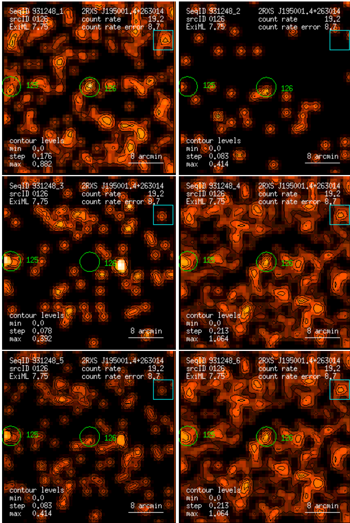
Figure 126: RASS 931248: detection 0126: band rate images, Gaussian filter: (1) PSPC channels 11 – 41, (2) 52 – 90, (3) 91 – 201, (4) 11 – 235, (5) 52 – 201, (6) 11 – 201. Broad band rates in counts/ks. Band rate contour levels in counts/ks/arcmin 2 .
