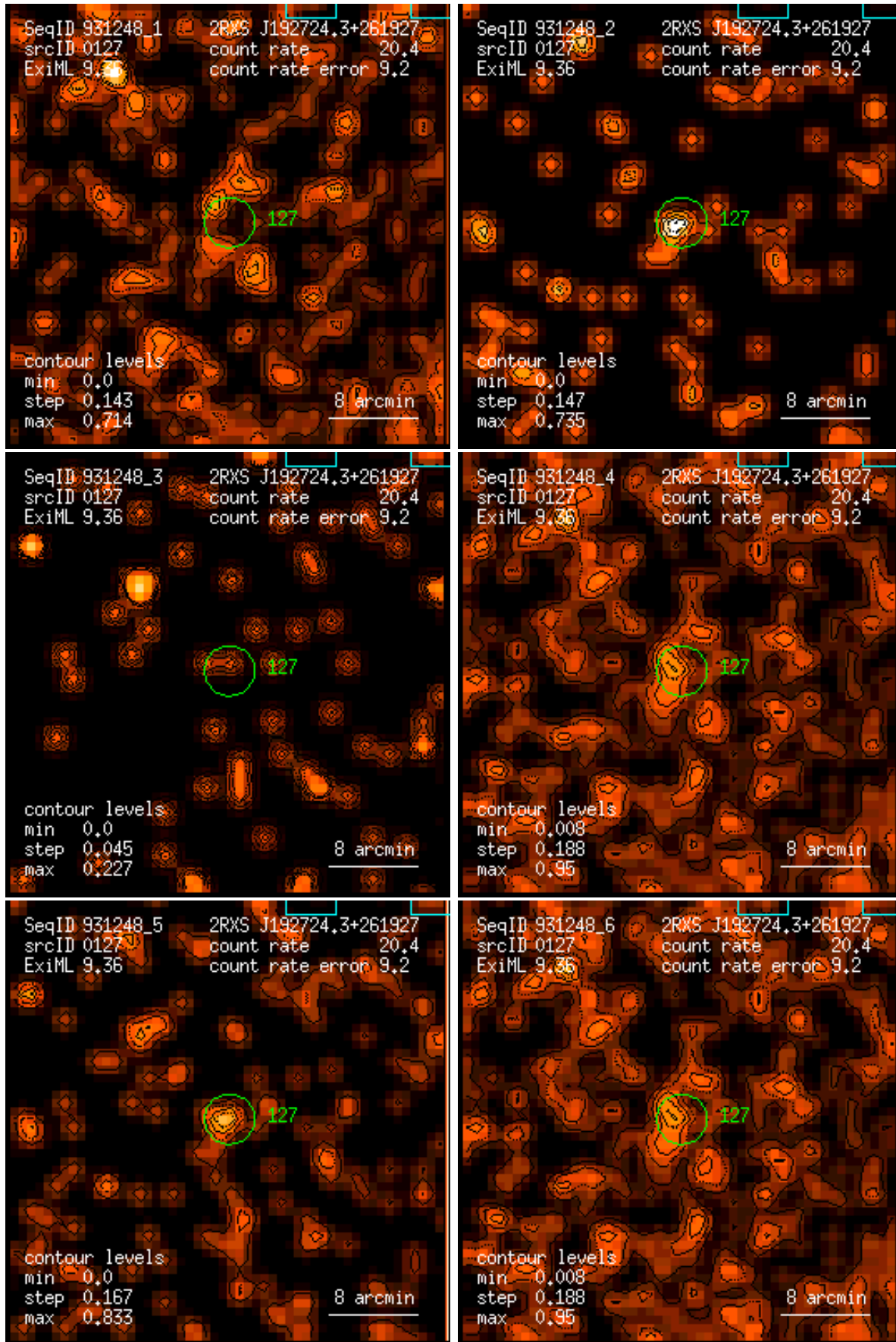
Figure 127: RASS 931248: detection 0127: band rate images, Gaussian filter: (1) PSPC channels 11 – 41, (2) 52 – 90, (3) 91 – 201, (4) 11 – 235, (5) 52 – 201, (6) 11 – 201. Broad band rates in counts/ks. Band rate contour levels in counts/ks/arcmin 2 .
