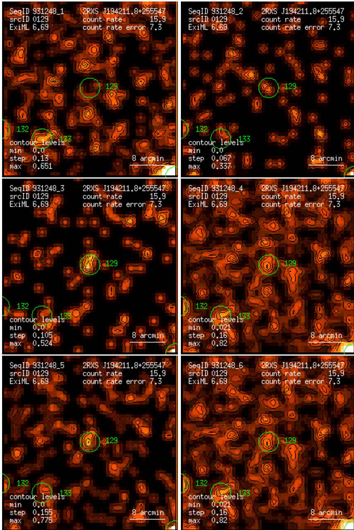
Figure 129: RASS 931248: detection 0129: band rate images, Gaussian filter: (1) PSPC channels 11 – 41, (2) 52 – 90, (3) 91 – 201, (4) 11 – 235, (5) 52 – 201, (6) 11 – 201. Broad band rates in counts/ks. Band rate contour levels in counts/ks/arcmin 2 .
