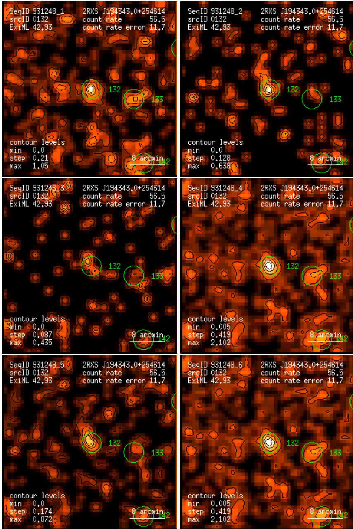
Figure 132: RASS 931248: detection 0132: band rate images, Gaussian filter: (1) PSPC channels 11 – 41, (2) 52 – 90, (3) 91 – 201, (4) 11 – 235, (5) 52 – 201, (6) 11 – 201. Broad band rates in counts/ks. Band rate contour levels in counts/ks/arcmin 2 .
