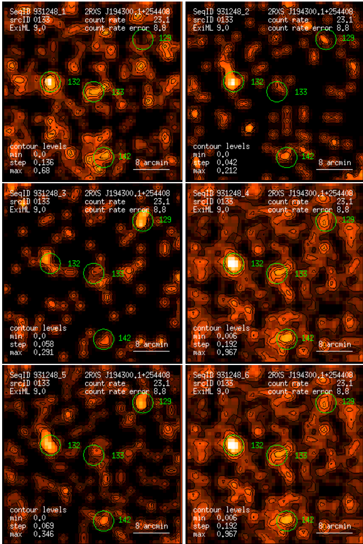
Figure 133: RASS 931248: detection 0133: band rate images, Gaussian filter: (1) PSPC channels 11 – 41, (2) 52 – 90, (3) 91 – 201, (4) 11 – 235, (5) 52 – 201, (6) 11 – 201. Broad band rates in counts/ks. Band rate contour levels in counts/ks/arcmin 2 .
