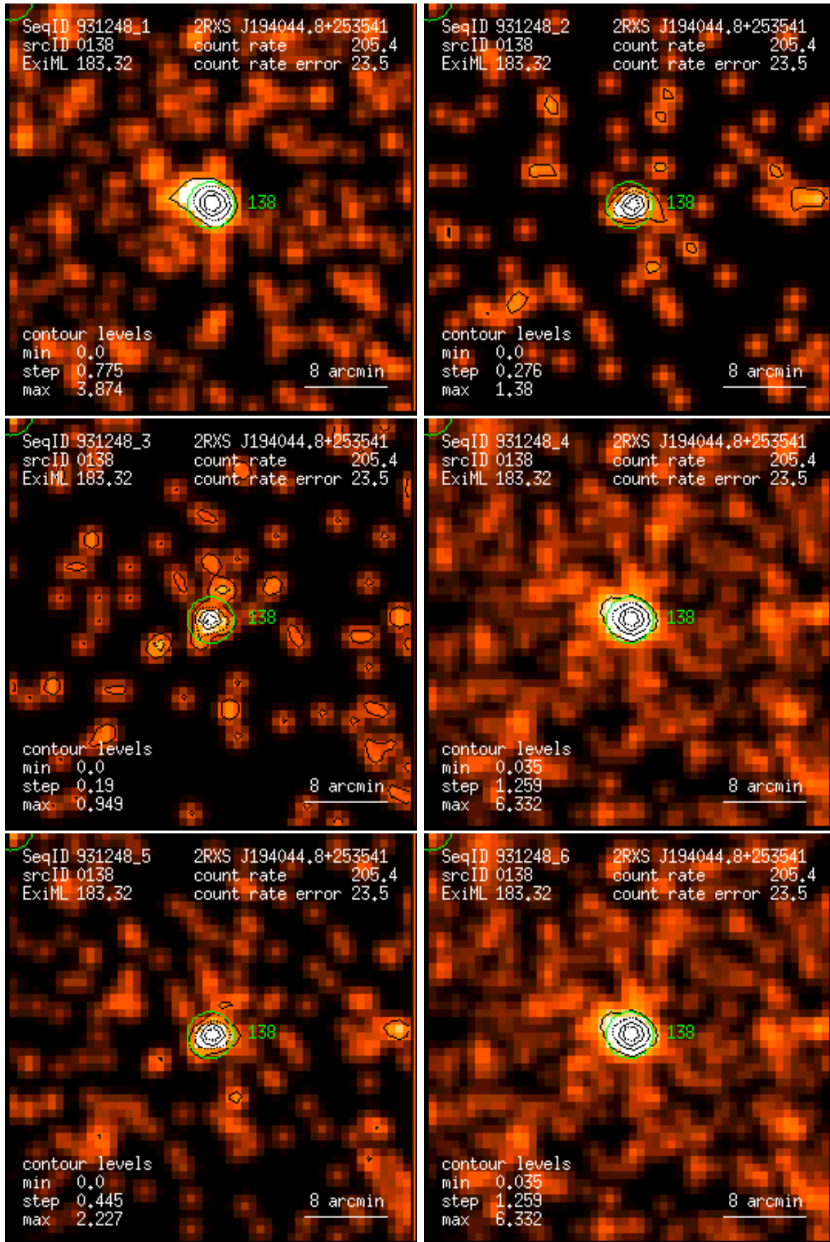
Figure 138: RASS 931248: detection 0138: band rate images, Gaussian filter: (1) PSPC channels 11 – 41, (2) 52 – 90, (3) 91 – 201, (4) 11 – 235, (5) 52 – 201, (6) 11 – 201. Broad band rates in counts/ks. Band rate contour levels in counts/ks/arcmin 2 .
