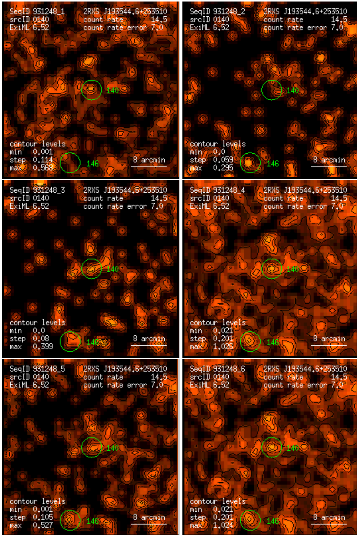
Figure 140: RASS 931248: detection 0140: band rate images, Gaussian filter: (1) PSPC channels 11 – 41, (2) 52 – 90, (3) 91 – 201, (4) 11 – 235, (5) 52 – 201, (6) 11 – 201. Broad band rates in counts/ks. Band rate contour levels in counts/ks/arcmin 2 .
