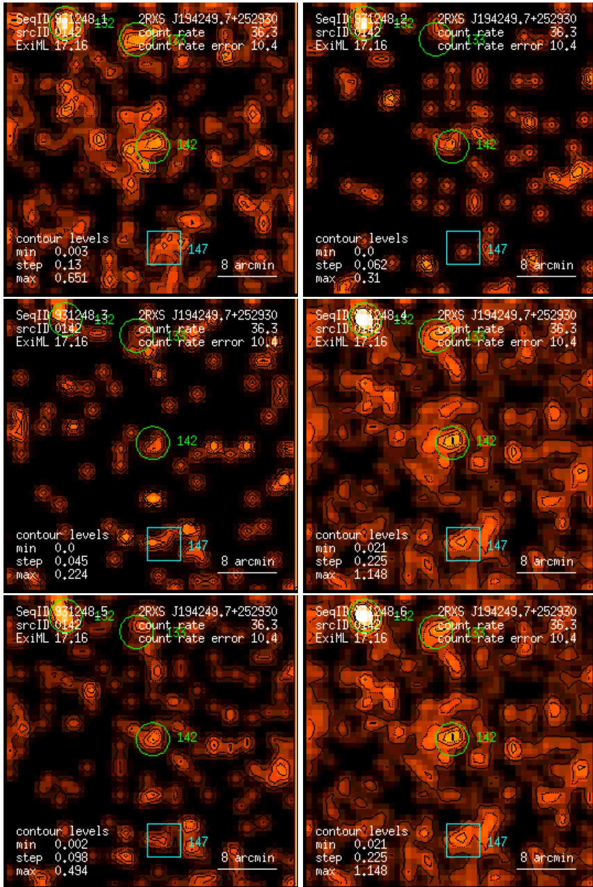
Figure 142: RASS 931248: detection 0142: band rate images, Gaussian filter: (1) PSPC channels 11 – 41, (2) 52 – 90, (3) 91 – 201, (4) 11 – 235, (5) 52 – 201, (6) 11 – 201. Broad band rates in counts/ks. Band rate contour levels in counts/ks/arcmin 2 .
