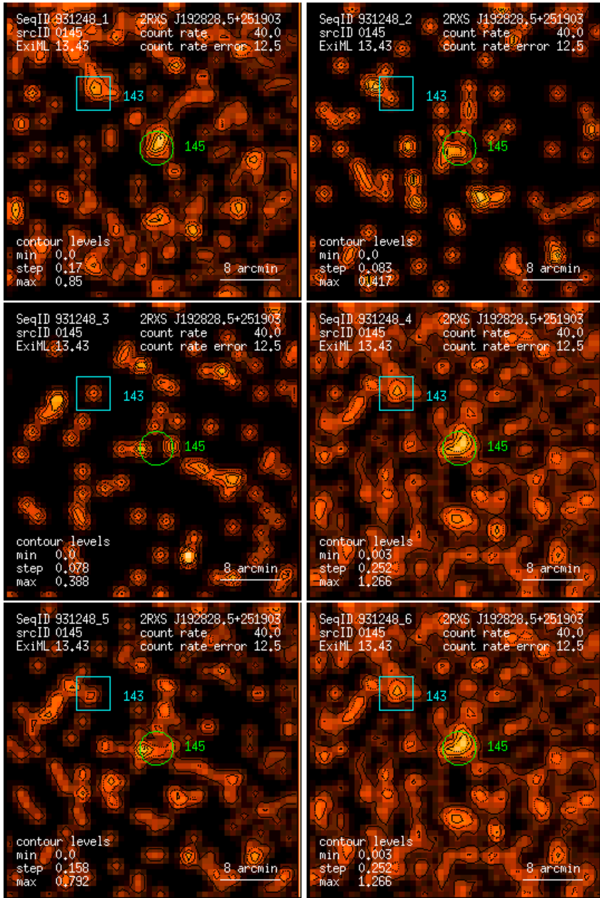
Figure 145: RASS 931248: detection 0145: band rate images, Gaussian filter: (1) PSPC channels 11 – 41, (2) 52 – 90, (3) 91 – 201, (4) 11 – 235, (5) 52 – 201, (6) 11 – 201. Broad band rates in counts/ks. Band rate contour levels in counts/ks/arcmin 2 .
