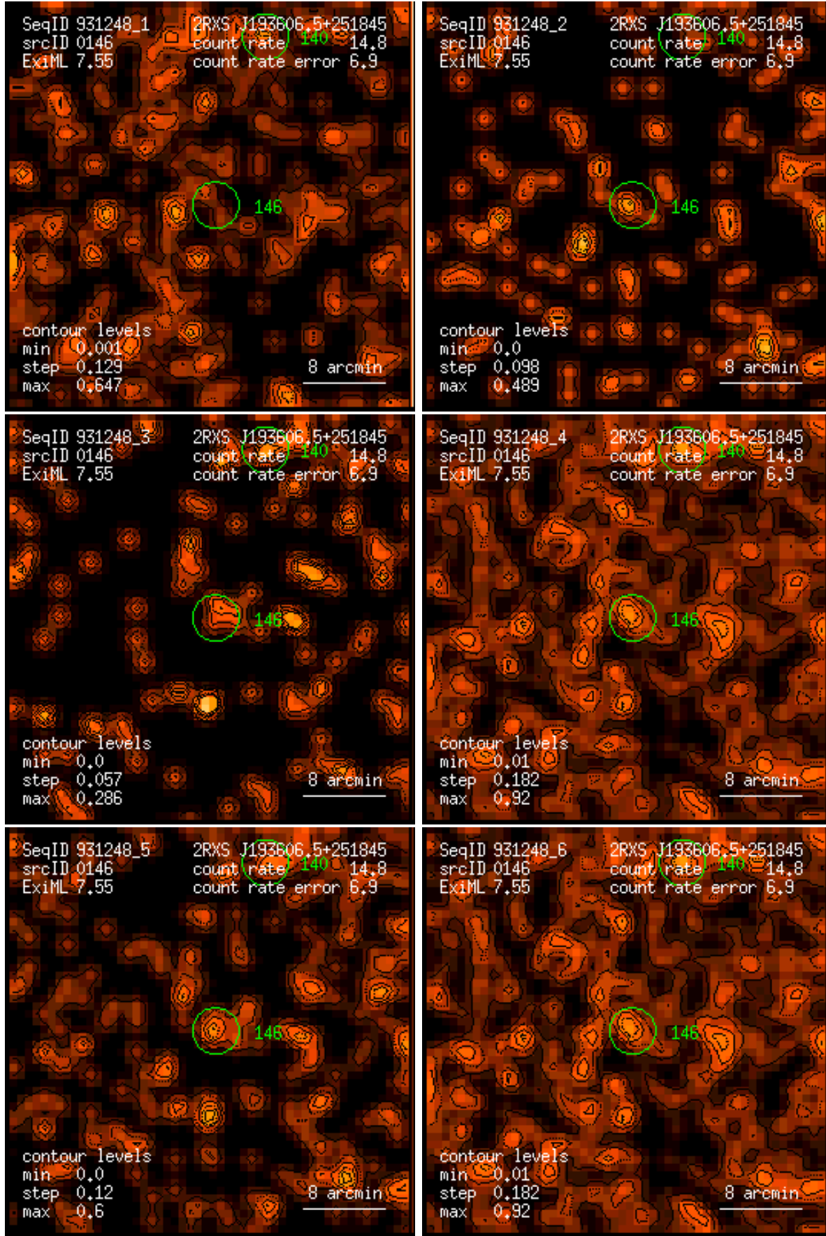
Figure 146: RASS 931248: detection 0146: band rate images, Gaussian filter: (1) PSPC channels 11 – 41, (2) 52 – 90, (3) 91 – 201, (4) 11 – 235, (5) 52 – 201, (6) 11 – 201. Broad band rates in counts/ks. Band rate contour levels in counts/ks/arcmin 2 .
