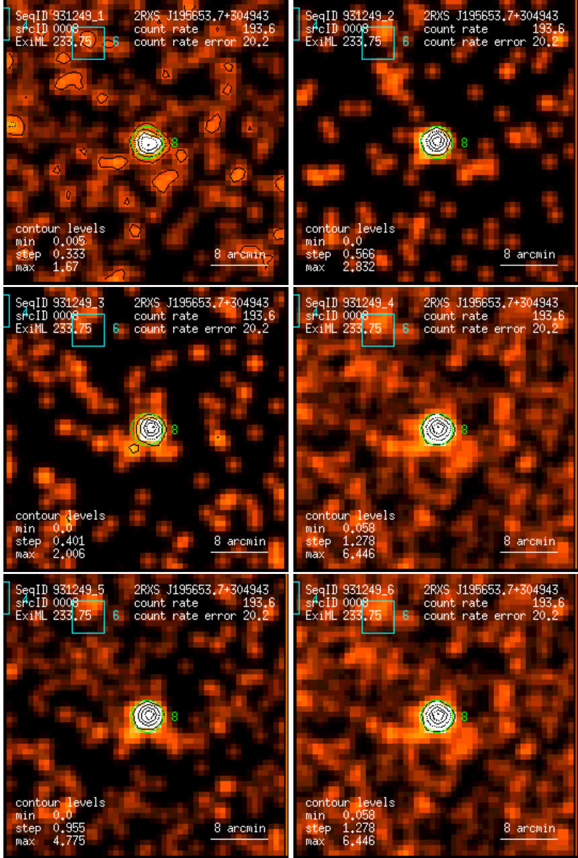
Figure 8: RASS 931249: detection 0008: band rate images, Gaussian filter: (1) PSPC channels 11 – 41, (2) 52 – 90, (3) 91 – 201, (4) 11 – 235, (5) 52 – 201, (6) 11 – 201. Broad band rates in counts/ks. Band rate contour levels in counts/ks/arcmin 2 .
