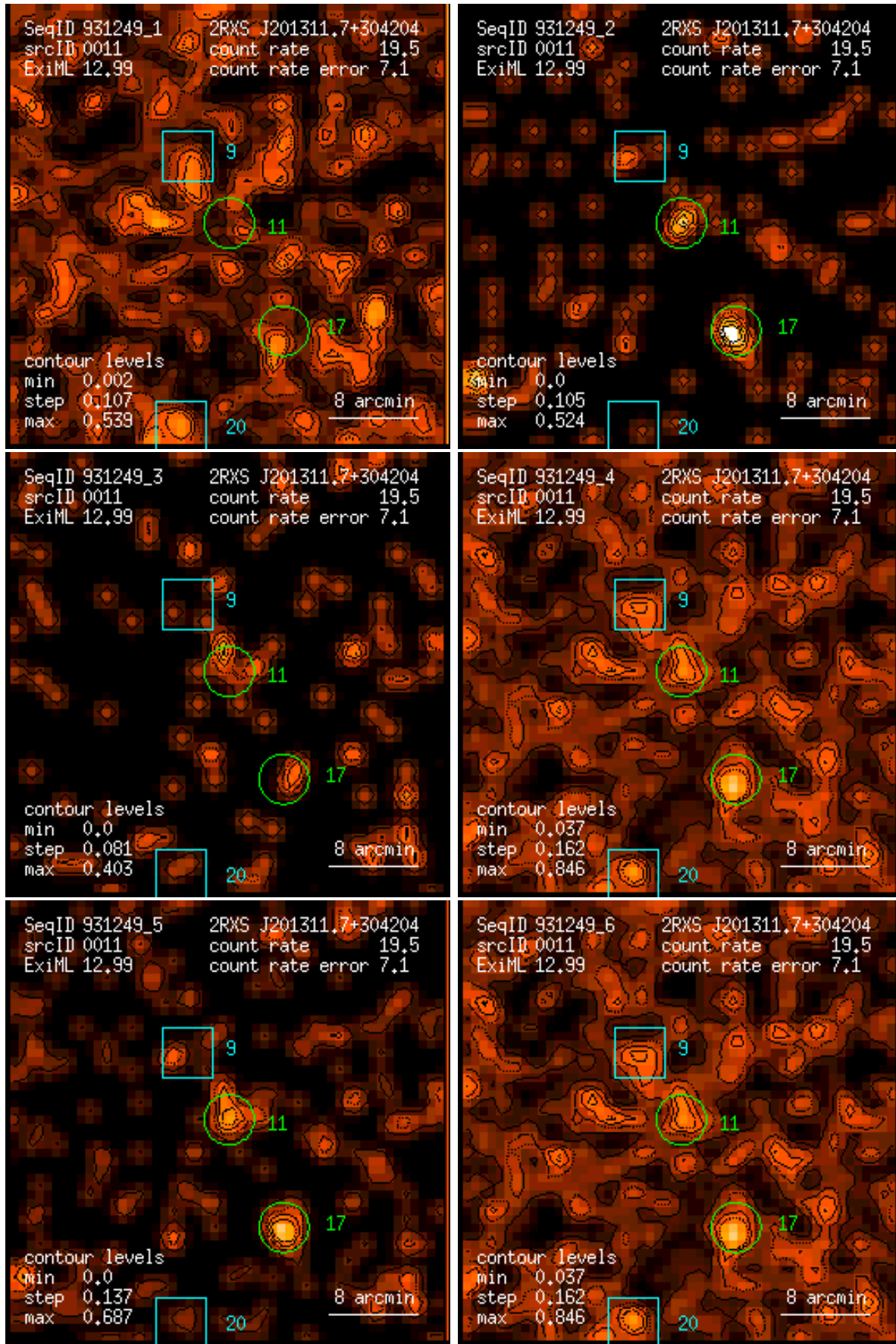
Figure 11: RASS 931249: detection 0011: band rate images, Gaussian filter: (1) PSPC channels 11 – 41, (2) 52 – 90, (3) 91 – 201, (4) 11 – 235, (5) 52 – 201, (6) 11 – 201. Broad band rates in counts/ks. Band rate contour levels in counts/ks/arcmin 2 .
