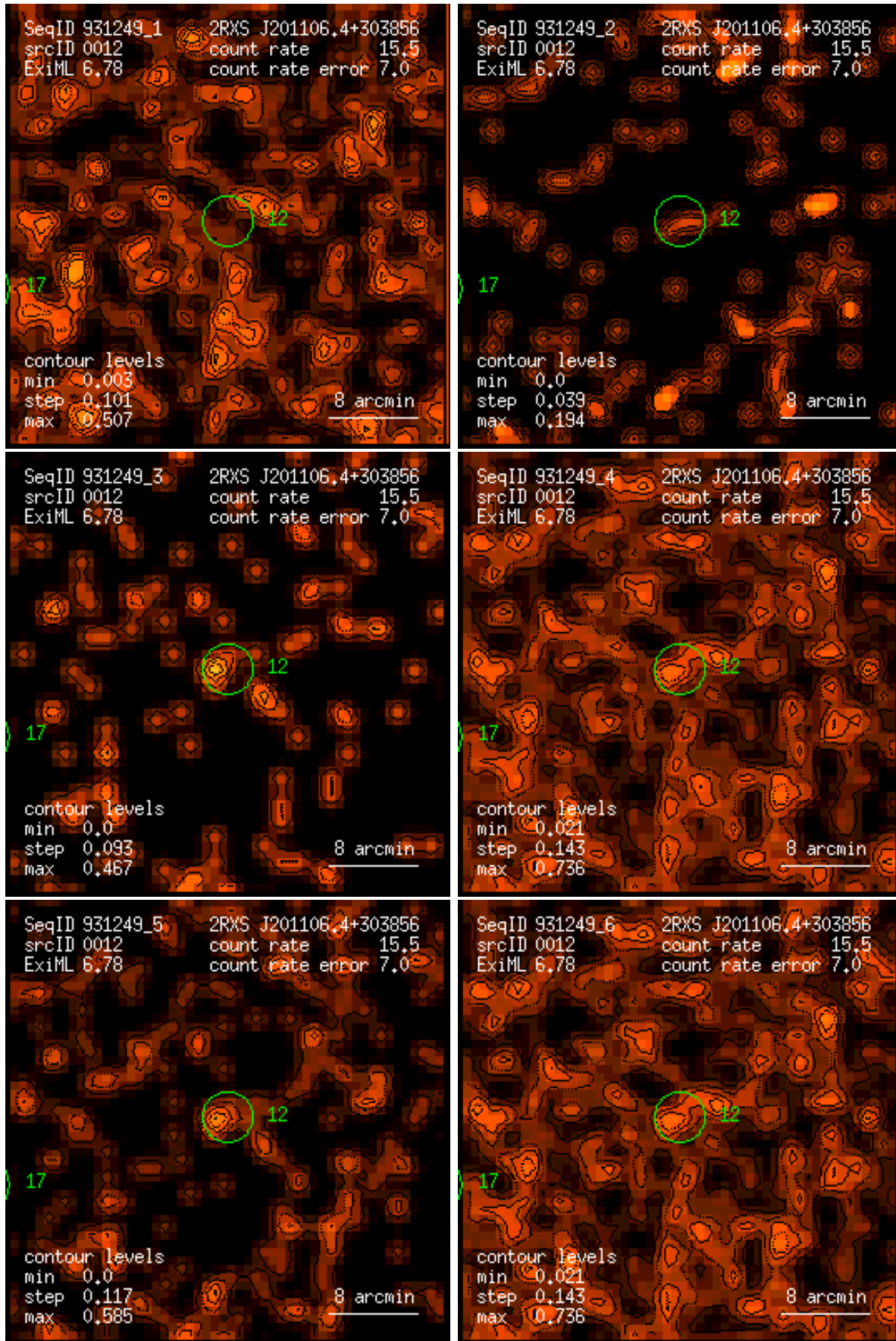
Figure 12: RASS 931249: detection 0012: band rate images, Gaussian filter: (1) PSPC channels 11 – 41, (2) 52 – 90, (3) 91 – 201, (4) 11 – 235, (5) 52 – 201, (6) 11 – 201. Broad band rates in counts/ks. Band rate contour levels in counts/ks/arcmin 2 .
