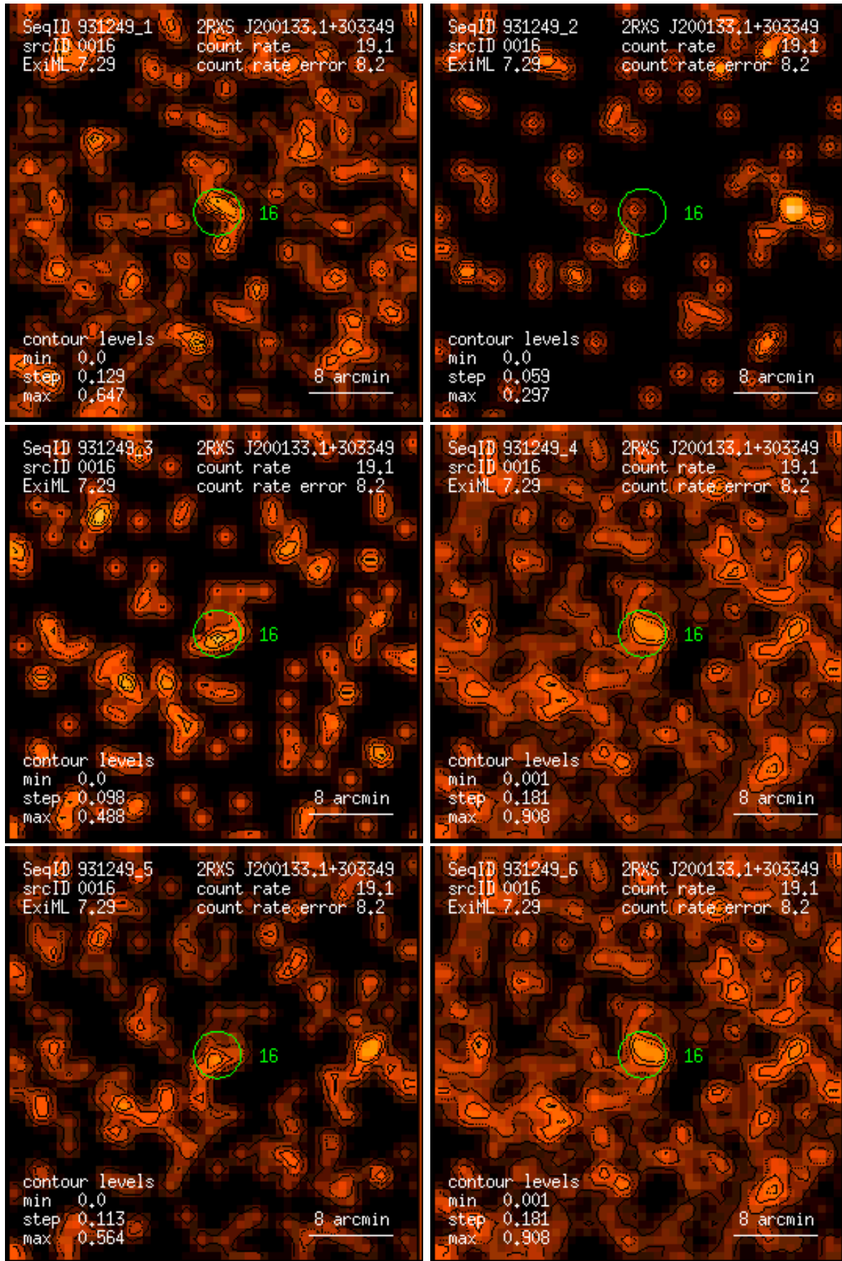
Figure 16: RASS 931249: detection 0016: band rate images, Gaussian filter: (1) PSPC channels 11 – 41, (2) 52 – 90, (3) 91 – 201, (4) 11 – 235, (5) 52 – 201, (6) 11 – 201. Broad band rates in counts/ks. Band rate contour levels in counts/ks/arcmin 2 .
