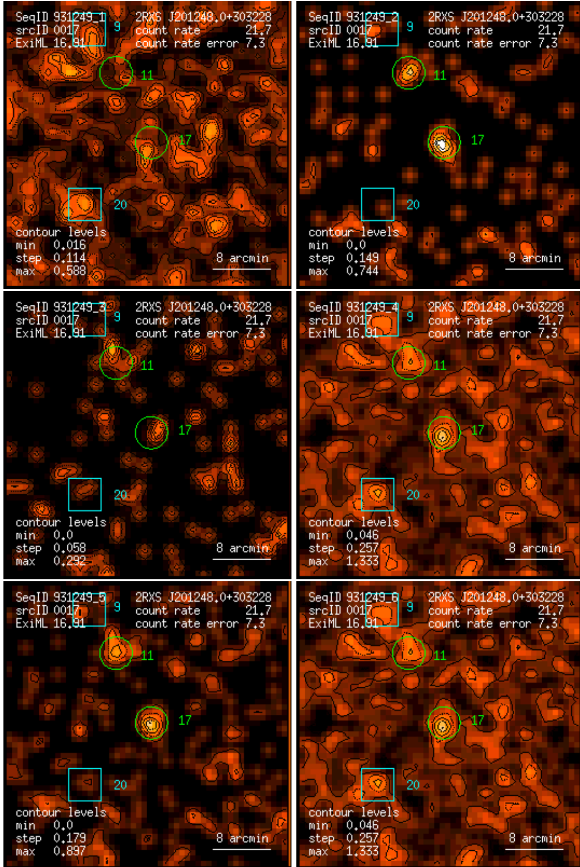
Figure 17: RASS 931249: detection 0017: band rate images, Gaussian filter: (1) PSPC channels 11 – 41, (2) 52 – 90, (3) 91 – 201, (4) 11 – 235, (5) 52 – 201, (6) 11 – 201. Broad band rates in counts/ks. Band rate contour levels in counts/ks/arcmin 2 .
