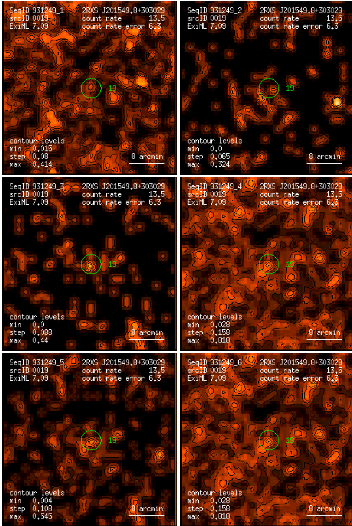
Figure 19: RASS 931249: detection 0019: band rate images, Gaussian filter: (1) PSPC channels 11 – 41, (2) 52 – 90, (3) 91 – 201, (4) 11 – 235, (5) 52 – 201, (6) 11 – 201. Broad band rates in counts/ks. Band rate contour levels in counts/ks/arcmin 2 .
