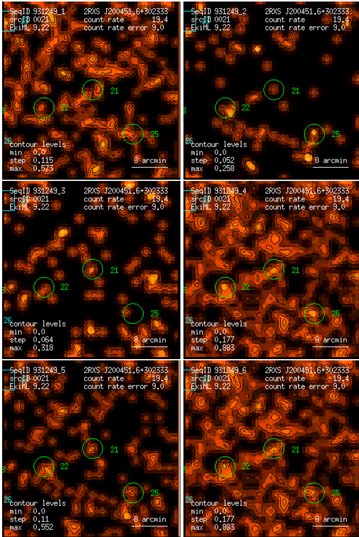
Figure 21: RASS 931249: detection 0021: band rate images, Gaussian filter: (1) PSPC channels 11 – 41, (2) 52 – 90, (3) 91 – 201, (4) 11 – 235, (5) 52 – 201, (6) 11 – 201. Broad band rates in counts/ks. Band rate contour levels in counts/ks/arcmin 2 .
