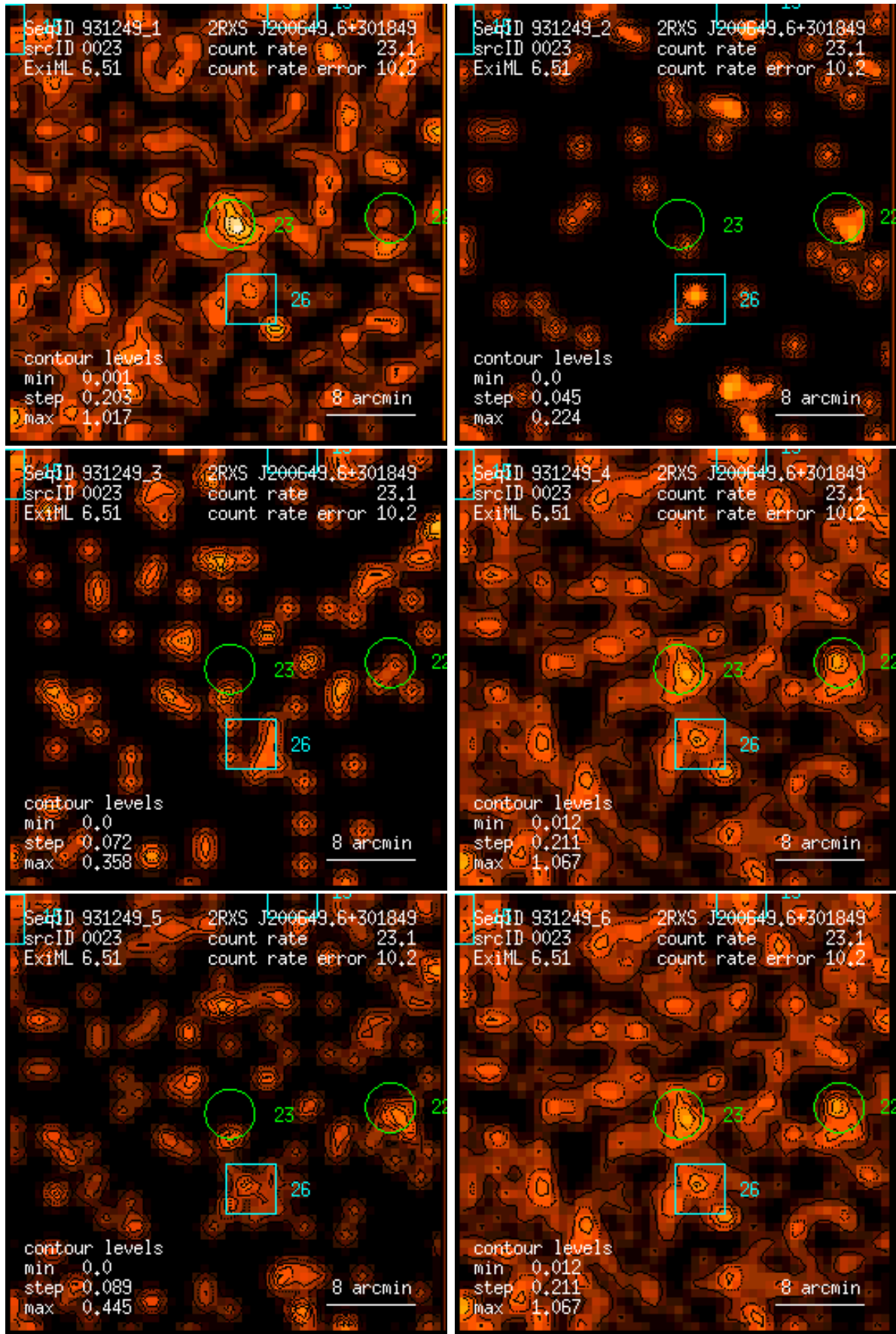
Figure 23: RASS 931249: detection 0023: band rate images, Gaussian filter: (1) PSPC channels 11 – 41, (2) 52 – 90, (3) 91 – 201, (4) 11 – 235, (5) 52 – 201, (6) 11 – 201. Broad band rates in counts/ks. Band rate contour levels in counts/ks/arcmin 2 .
