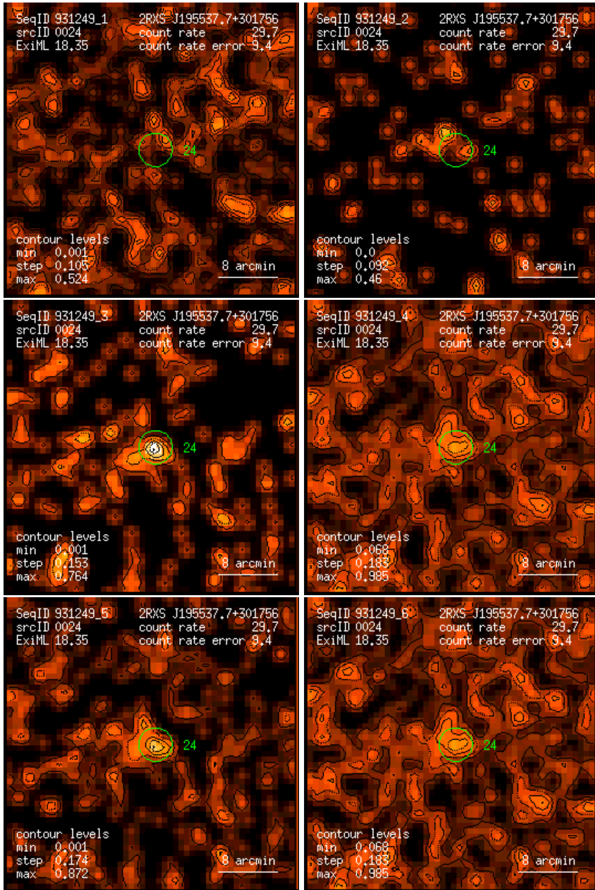
Figure 24: RASS 931249: detection 0024: band rate images, Gaussian filter: (1) PSPC channels 11 – 41, (2) 52 – 90, (3) 91 – 201, (4) 11 – 235, (5) 52 – 201, (6) 11 – 201. Broad band rates in counts/ks. Band rate contour levels in counts/ks/arcmin 2 .
