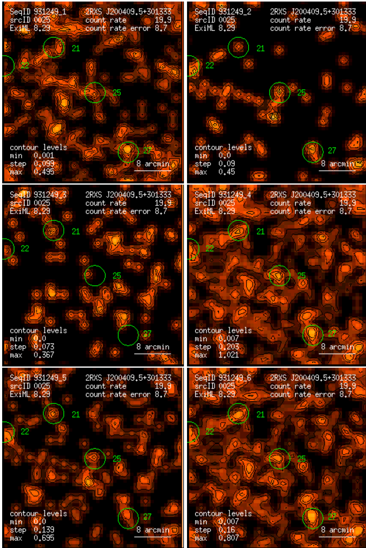
Figure 25: RASS 931249: detection 0025: band rate images, Gaussian filter: (1) PSPC channels 11 – 41, (2) 52 – 90, (3) 91 – 201, (4) 11 – 235, (5) 52 – 201, (6) 11 – 201. Broad band rates in counts/ks. Band rate contour levels in counts/ks/arcmin 2 .
