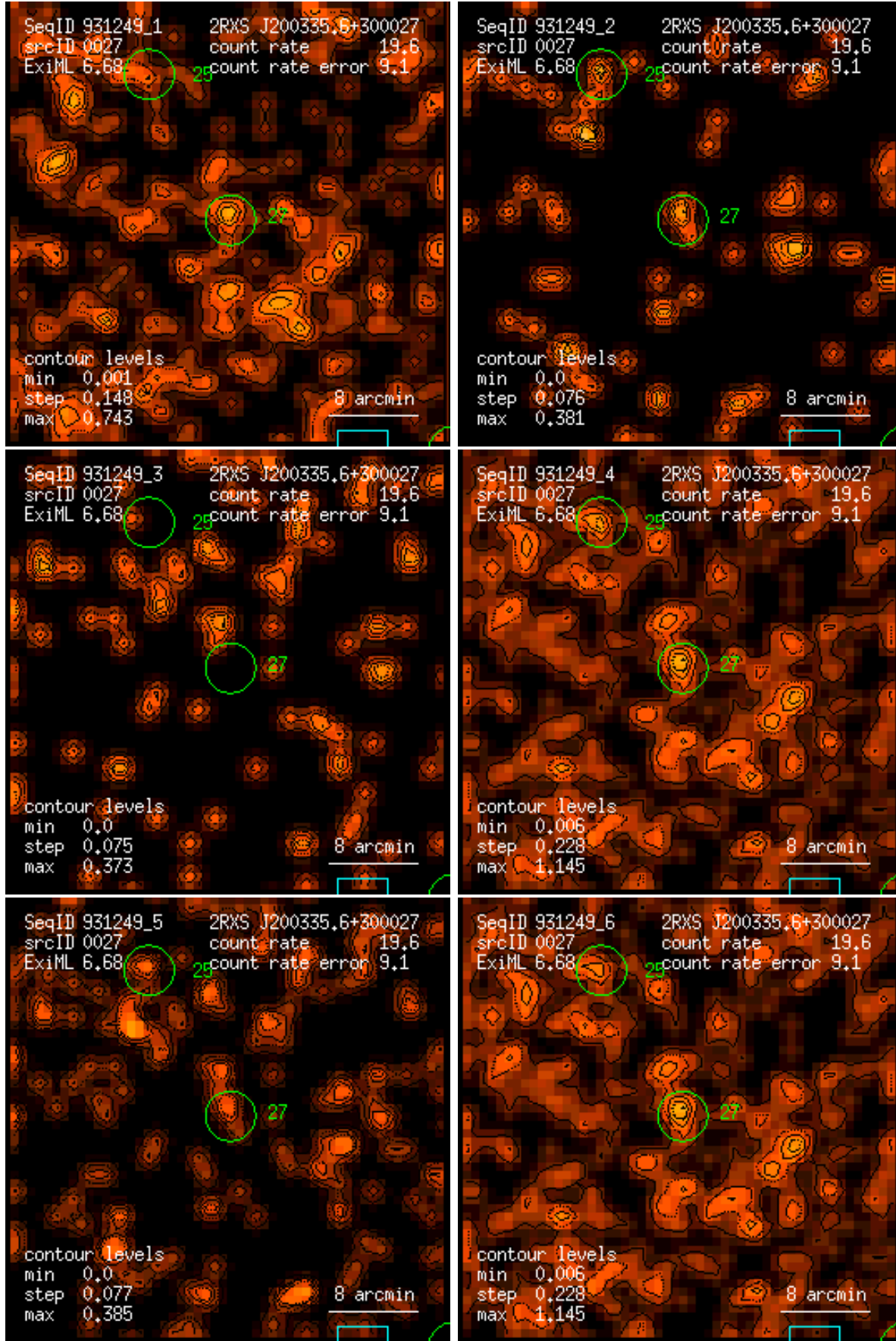
Figure 27: RASS 931249: detection 0027: band rate images, Gaussian filter: (1) PSPC channels 11 – 41, (2) 52 – 90, (3) 91 – 201, (4) 11 – 235, (5) 52 – 201, (6) 11 – 201. Broad band rates in counts/ks. Band rate contour levels in counts/ks/arcmin 2 .
