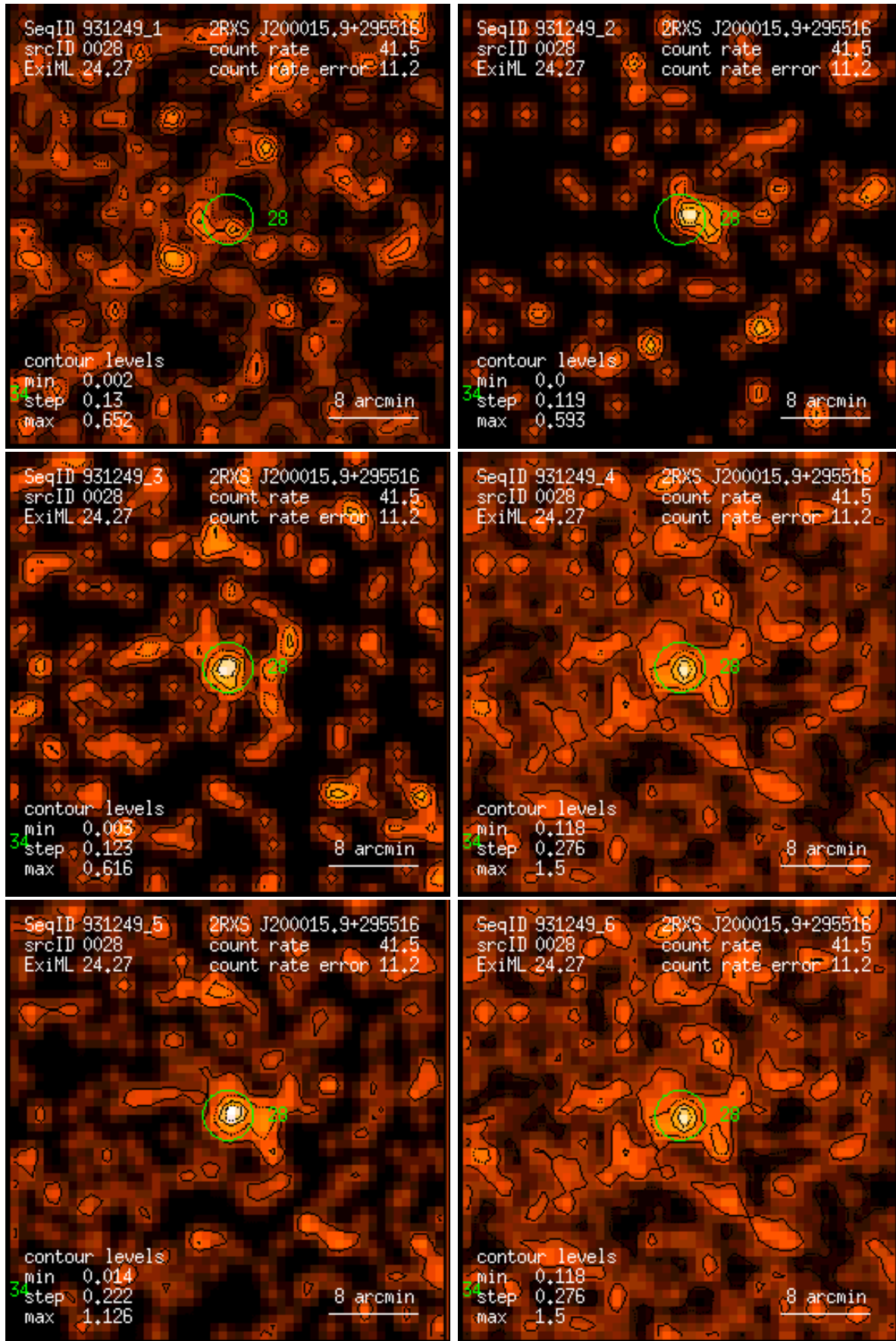
Figure 28: RASS 931249: detection 0028: band rate images, Gaussian filter: (1) PSPC channels 11 – 41, (2) 52 – 90, (3) 91 – 201, (4) 11 – 235, (5) 52 – 201, (6) 11 – 201. Broad band rates in counts/ks. Band rate contour levels in counts/ks/arcmin 2 .
