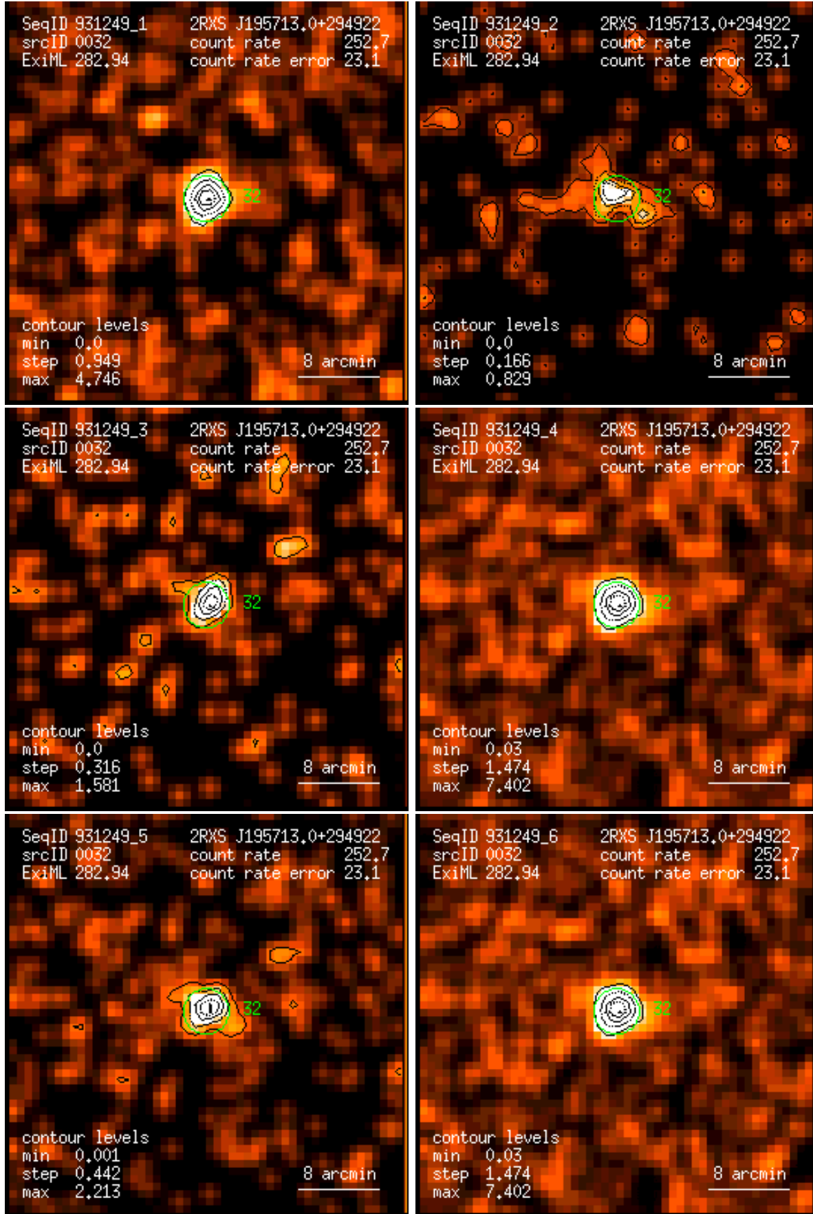
Figure 32: RASS 931249: detection 0032: band rate images, Gaussian filter: (1) PSPC channels 11 – 41, (2) 52 – 90, (3) 91 – 201, (4) 11 – 235, (5) 52 – 201, (6) 11 – 201. Broad band rates in counts/ks. Band rate contour levels in counts/ks/arcmin 2 .
