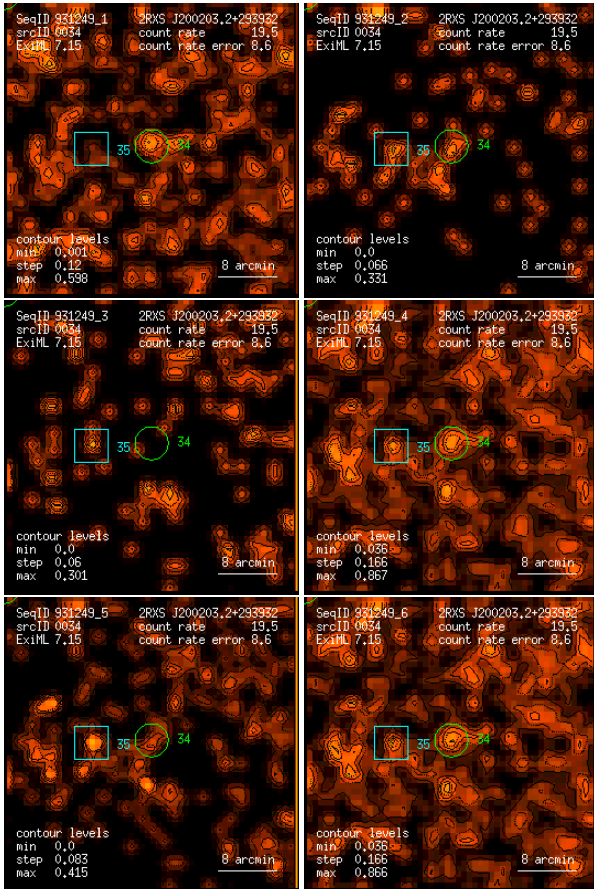
Figure 34: RASS 931249: detection 0034: band rate images, Gaussian filter: (1) PSPC channels 11 – 41, (2) 52 – 90, (3) 91 – 201, (4) 11 – 235, (5) 52 – 201, (6) 11 – 201. Broad band rates in counts/ks. Band rate contour levels in counts/ks/arcmin 2 .
