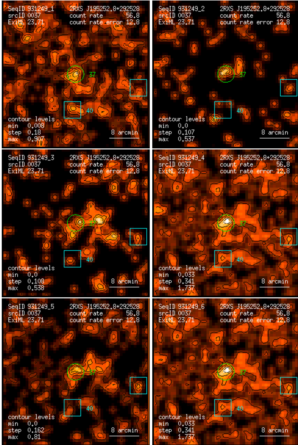
Figure 37: RASS 931249: detection 0037: band rate images, Gaussian filter: (1) PSPC channels 11 – 41, (2) 52 – 90, (3) 91 – 201, (4) 11 – 235, (5) 52 – 201, (6) 11 – 201. Broad band rates in counts/ks. Band rate contour levels in counts/ks/arcmin 2 .
