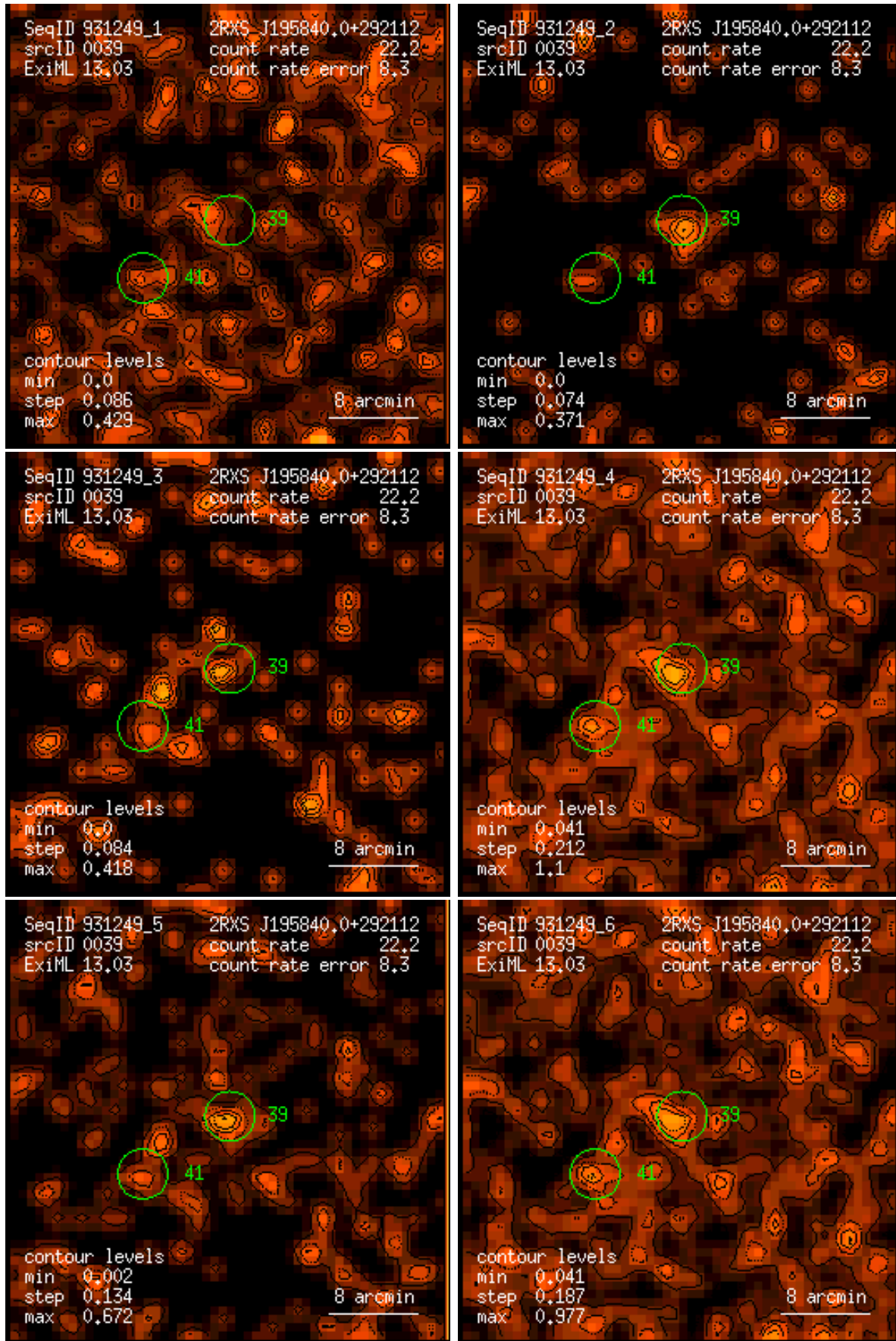
Figure 39: RASS 931249: detection 0039: band rate images, Gaussian filter: (1) PSPC channels 11 – 41, (2) 52 – 90, (3) 91 – 201, (4) 11 – 235, (5) 52 – 201, (6) 11 – 201. Broad band rates in counts/ks. Band rate contour levels in counts/ks/arcmin 2 .
