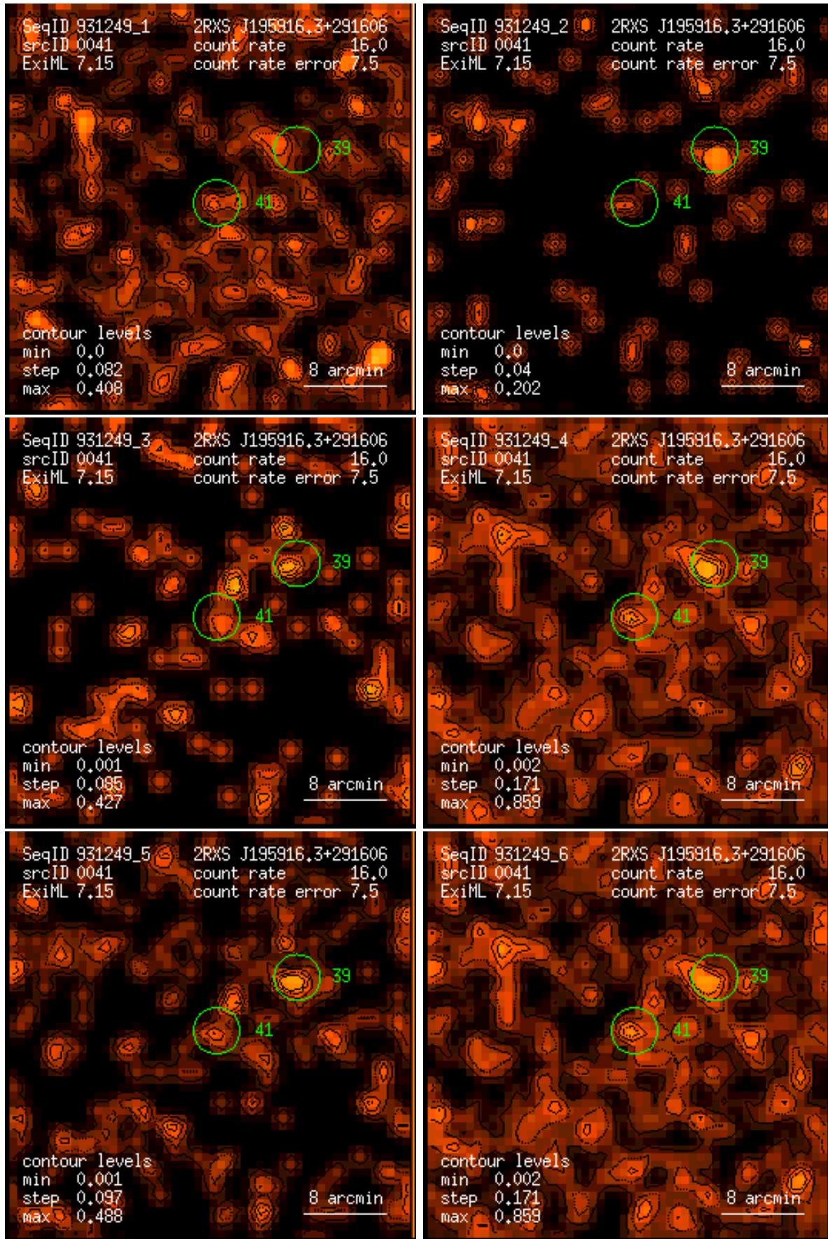
Figure 41: RASS 931249: detection 0041: band rate images, Gaussian filter: (1) PSPC channels 11 – 41, (2) 52 – 90, (3) 91 – 201, (4) 11 – 235, (5) 52 – 201, (6) 11 – 201. Broad band rates in counts/ks. Band rate contour levels in counts/ks/arcmin 2 .
