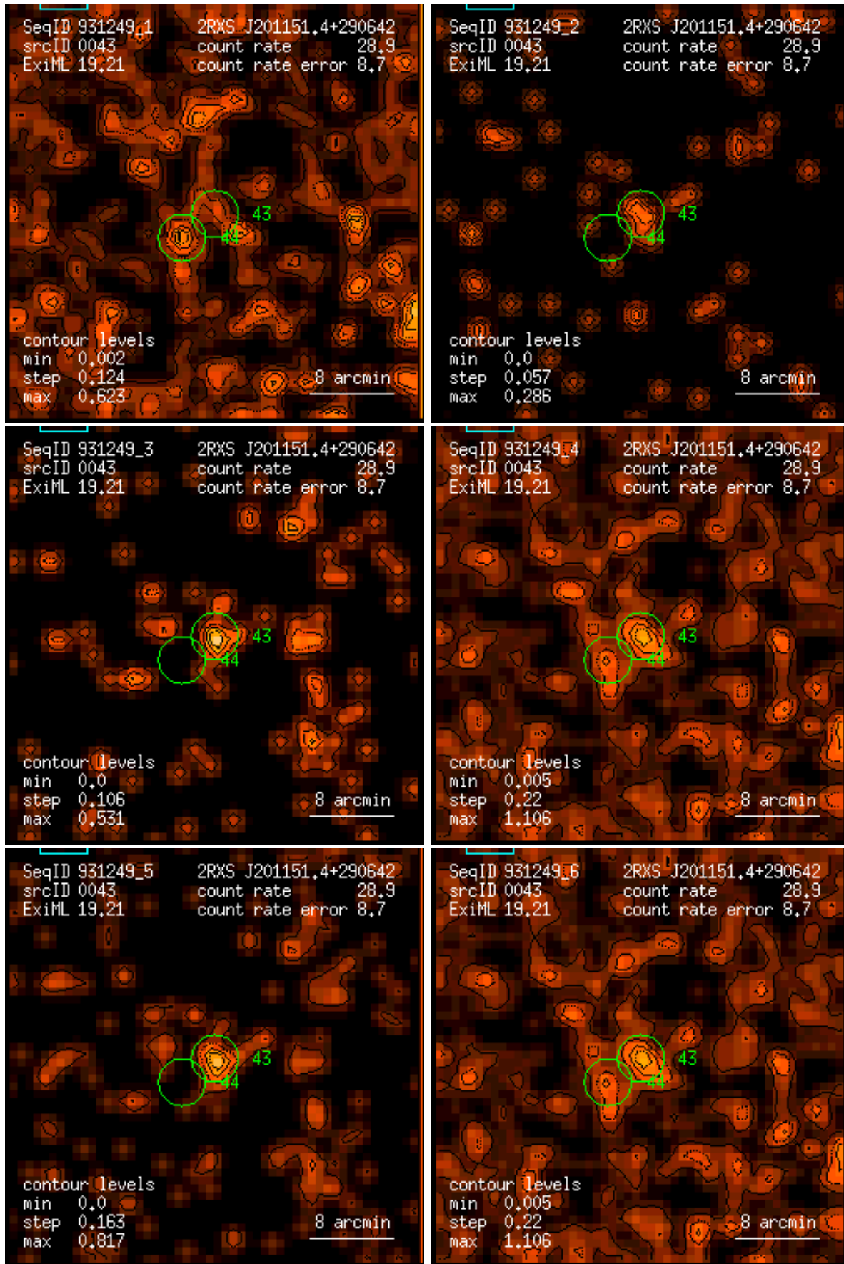
Figure 43: RASS 931249: detection 0043: band rate images, Gaussian filter: (1) PSPC channels 11 – 41, (2) 52 – 90, (3) 91 – 201, (4) 11 – 235, (5) 52 – 201, (6) 11 – 201. Broad band rates in counts/ks. Band rate contour levels in counts/ks/arcmin 2 .
