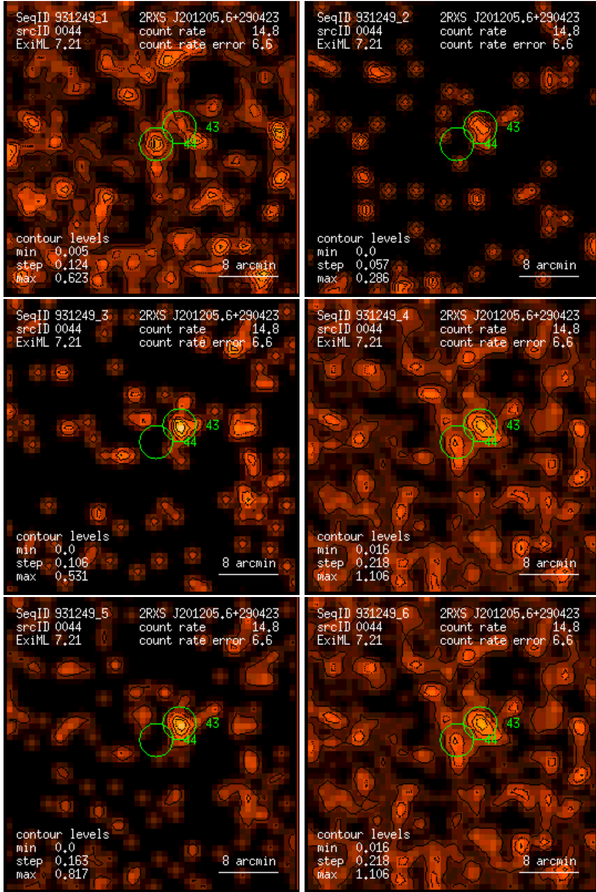
Figure 44: RASS 931249: detection 0044: band rate images, Gaussian filter: (1) PSPC channels 11 – 41, (2) 52 – 90, (3) 91 – 201, (4) 11 – 235, (5) 52 – 201, (6) 11 – 201. Broad band rates in counts/ks. Band rate contour levels in counts/ks/arcmin 2 .
