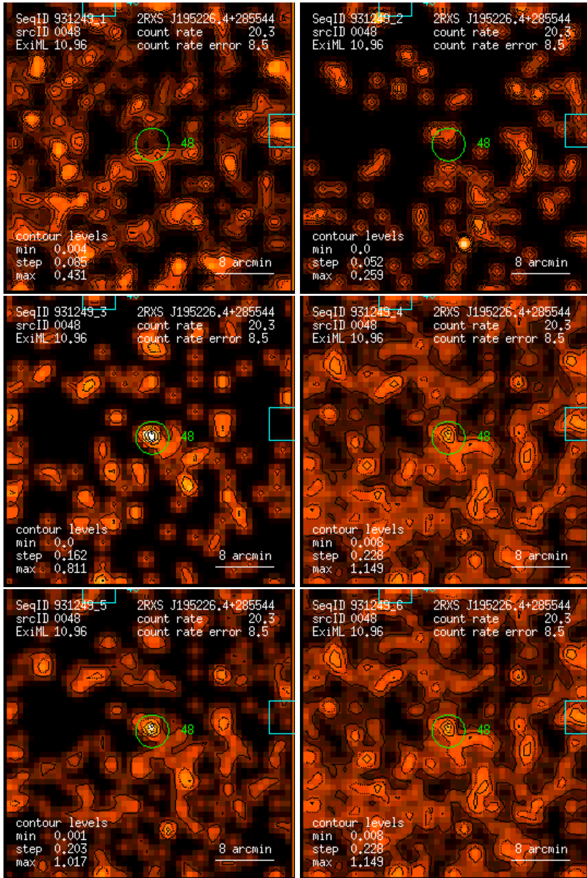
Figure 48: RASS 931249: detection 0048: band rate images, Gaussian filter: (1) PSPC channels 11 – 41, (2) 52 – 90, (3) 91 – 201, (4) 11 – 235, (5) 52 – 201, (6) 11 – 201. Broad band rates in counts/ks. Band rate contour levels in counts/ks/arcmin 2 .
