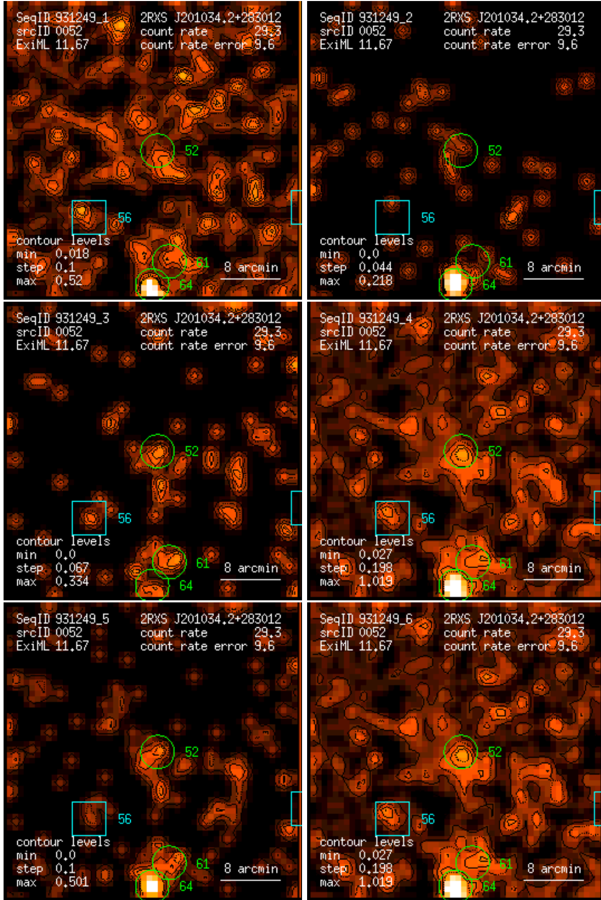
Figure 52: RASS 931249: detection 0052: band rate images, Gaussian filter: (1) PSPC channels 11 – 41, (2) 52 – 90, (3) 91 – 201, (4) 11 – 235, (5) 52 – 201, (6) 11 – 201. Broad band rates in counts/ks. Band rate contour levels in counts/ks/arcmin 2 .
