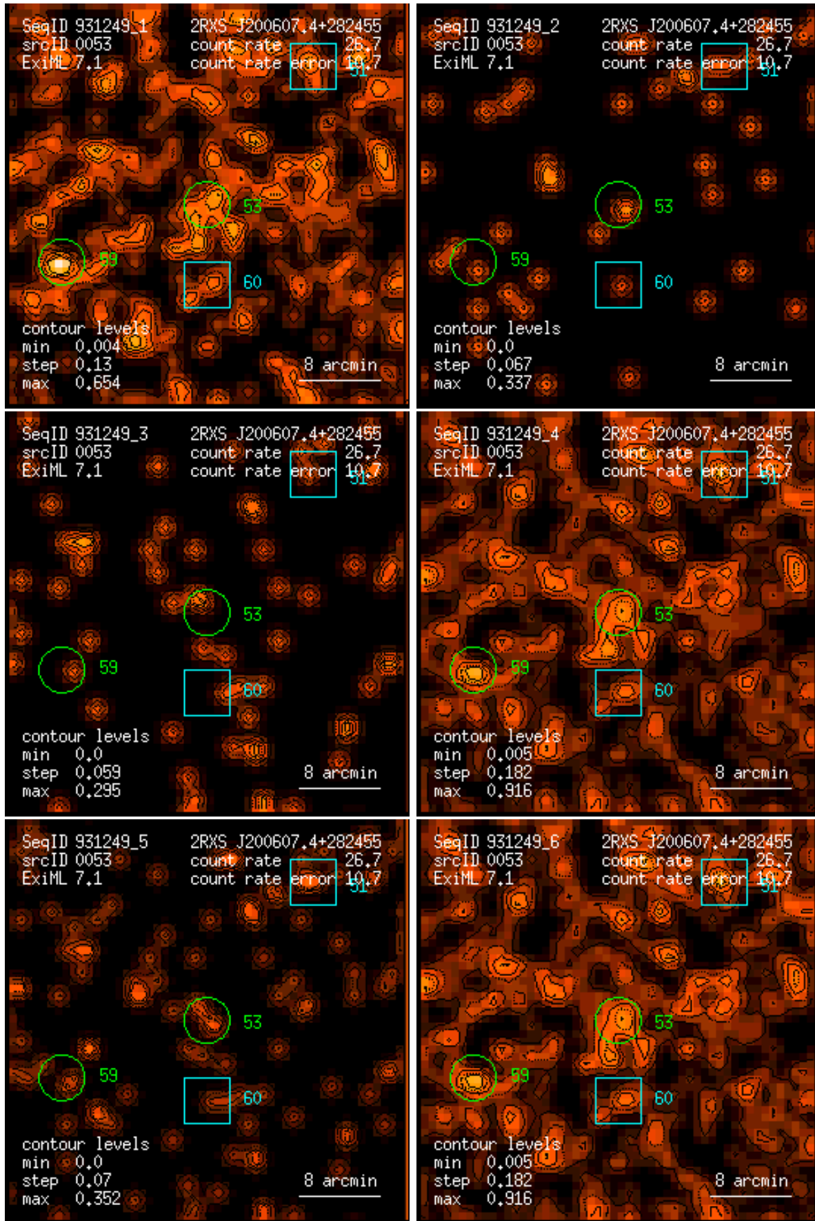
Figure 53: RASS 931249: detection 0053: band rate images, Gaussian filter: (1) PSPC channels 11 – 41, (2) 52 – 90, (3) 91 – 201, (4) 11 – 235, (5) 52 – 201, (6) 11 – 201. Broad band rates in counts/ks. Band rate contour levels in counts/ks/arcmin 2 .
