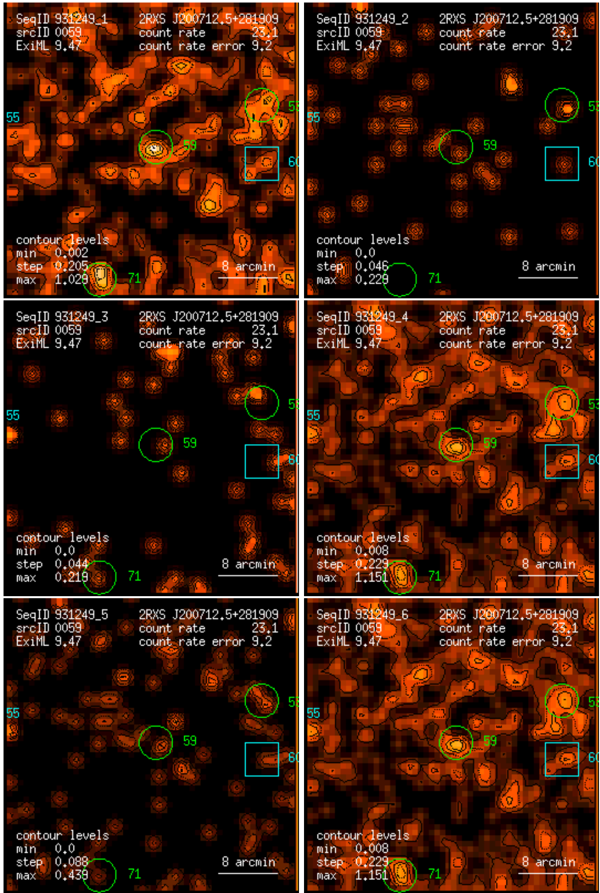
Figure 59: RASS 931249: detection 0059: band rate images, Gaussian filter: (1) PSPC channels 11 – 41, (2) 52 – 90, (3) 91 – 201, (4) 11 – 235, (5) 52 – 201, (6) 11 – 201. Broad band rates in counts/ks. Band rate contour levels in counts/ks/arcmin 2 .
