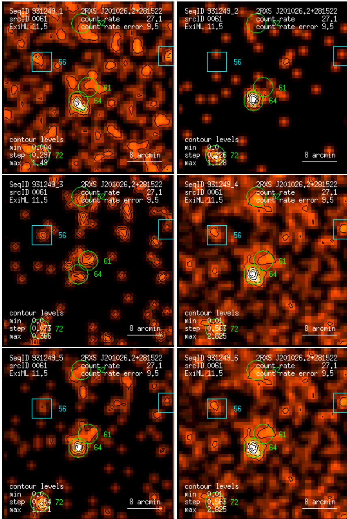
Figure 61: RASS 931249: detection 0061: band rate images, Gaussian filter: (1) PSPC channels 11 – 41, (2) 52 – 90, (3) 91 – 201, (4) 11 – 235, (5) 52 – 201, (6) 11 – 201. Broad band rates in counts/ks. Band rate contour levels in counts/ks/arcmin 2 .
