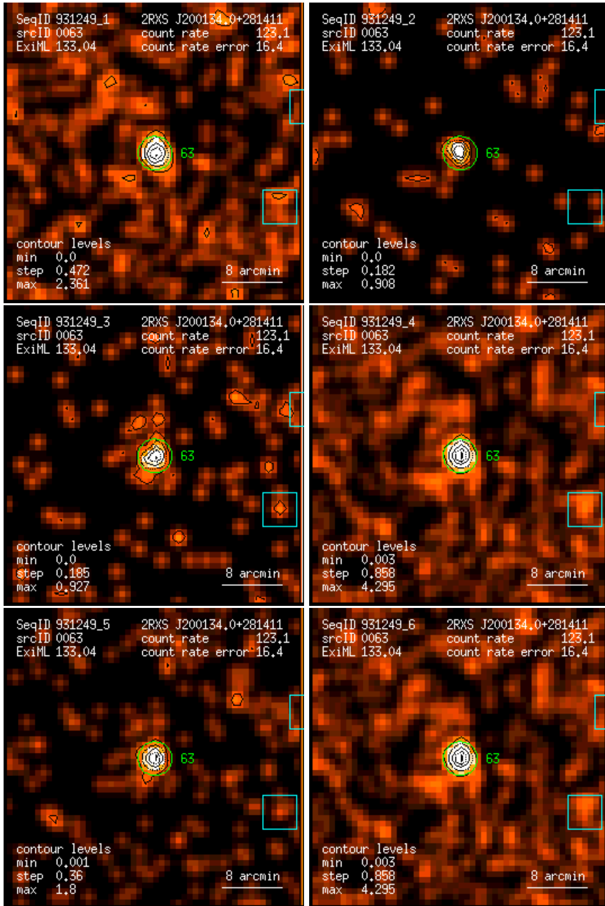
Figure 63: RASS 931249: detection 0063: band rate images, Gaussian filter: (1) PSPC channels 11 – 41, (2) 52 – 90, (3) 91 – 201, (4) 11 – 235, (5) 52 – 201, (6) 11 – 201. Broad band rates in counts/ks. Band rate contour levels in counts/ks/arcmin 2 .
