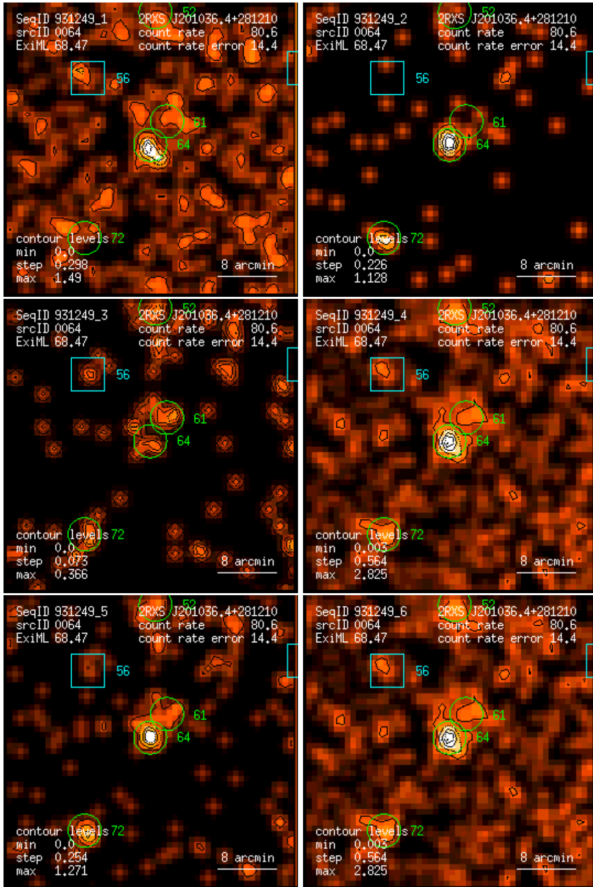
Figure 64: RASS 931249: detection 0064: band rate images, Gaussian filter: (1) PSPC channels 11 – 41, (2) 52 – 90, (3) 91 – 201, (4) 11 – 235, (5) 52 – 201, (6) 11 – 201. Broad band rates in counts/ks. Band rate contour levels in counts/ks/arcmin 2 .
