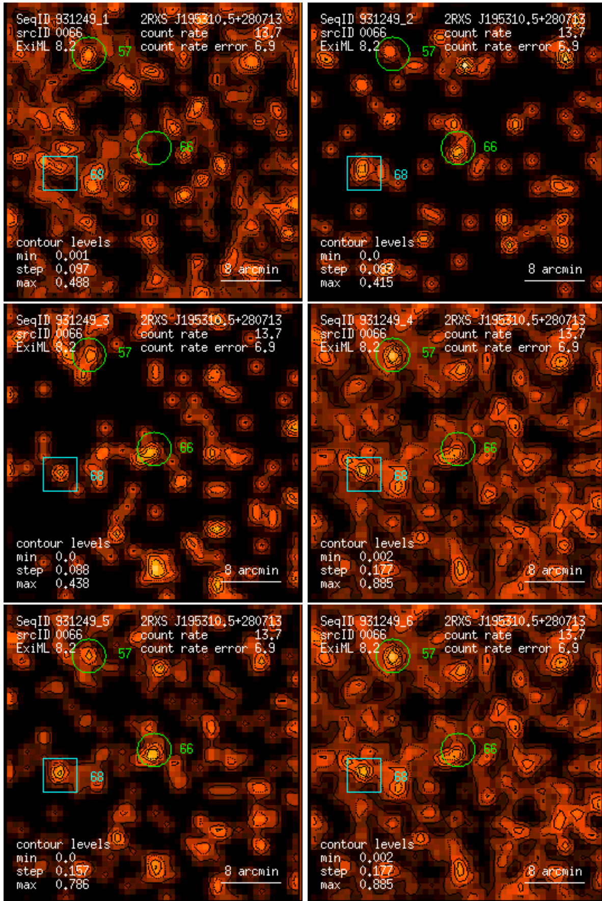
Figure 66: RASS 931249: detection 0066: band rate images, Gaussian filter: (1) PSPC channels 11 – 41, (2) 52 – 90, (3) 91 – 201, (4) 11 – 235, (5) 52 – 201, (6) 11 – 201. Broad band rates in counts/ks. Band rate contour levels in counts/ks/arcmin 2 .
