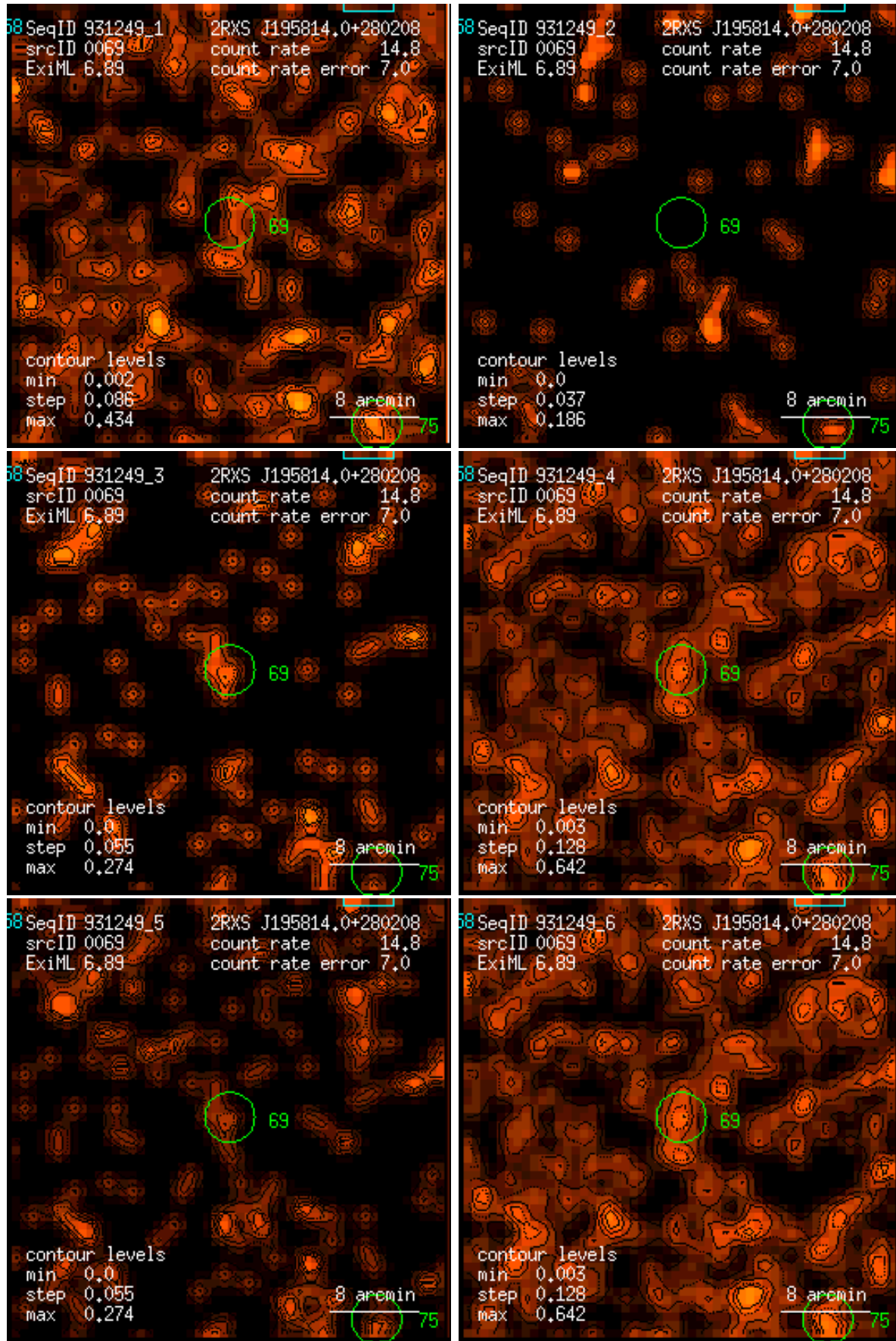
Figure 69: RASS 931249: detection 0069: band rate images, Gaussian filter: (1) PSPC channels 11 – 41, (2) 52 – 90, (3) 91 – 201, (4) 11 – 235, (5) 52 – 201, (6) 11 – 201. Broad band rates in counts/ks. Band rate contour levels in counts/ks/arcmin 2 .
