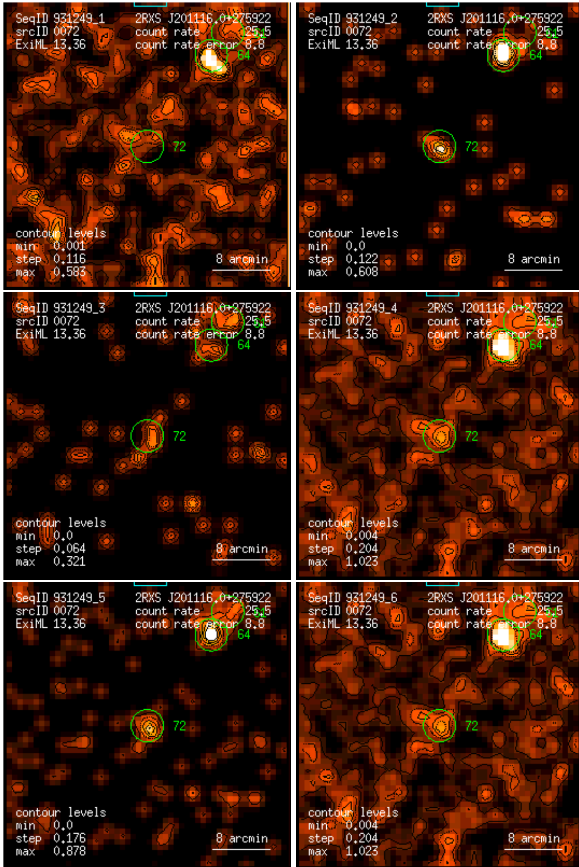
Figure 72: RASS 931249: detection 0072: band rate images, Gaussian filter: (1) PSPC channels 11 – 41, (2) 52 – 90, (3) 91 – 201, (4) 11 – 235, (5) 52 – 201, (6) 11 – 201. Broad band rates in counts/ks. Band rate contour levels in counts/ks/arcmin 2 .
