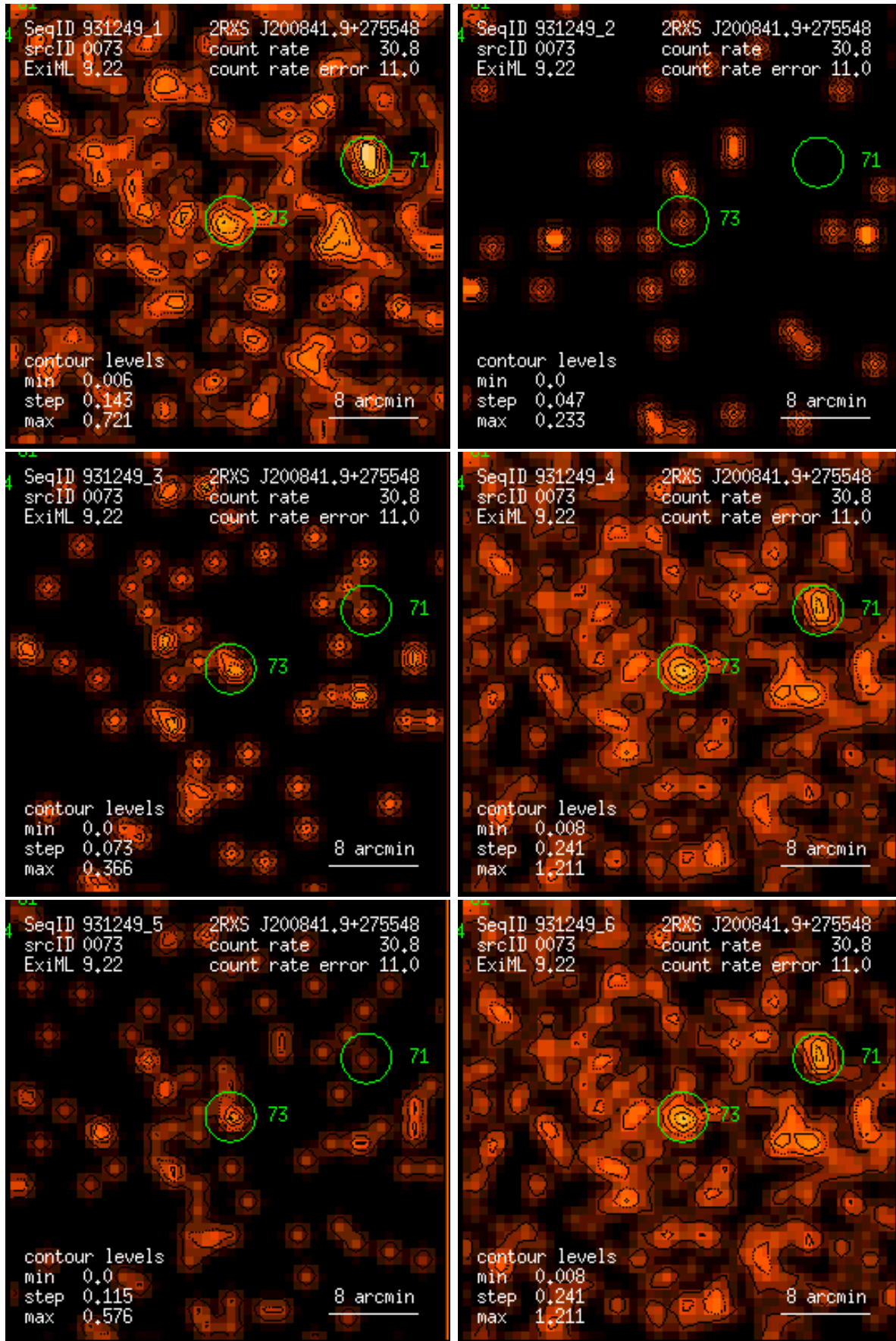
Figure 73: RASS 931249: detection 0073: band rate images, Gaussian filter: (1) PSPC channels 11 – 41, (2) 52 – 90, (3) 91 – 201, (4) 11 – 235, (5) 52 – 201, (6) 11 – 201. Broad band rates in counts/ks. Band rate contour levels in counts/ks/arcmin 2 .
