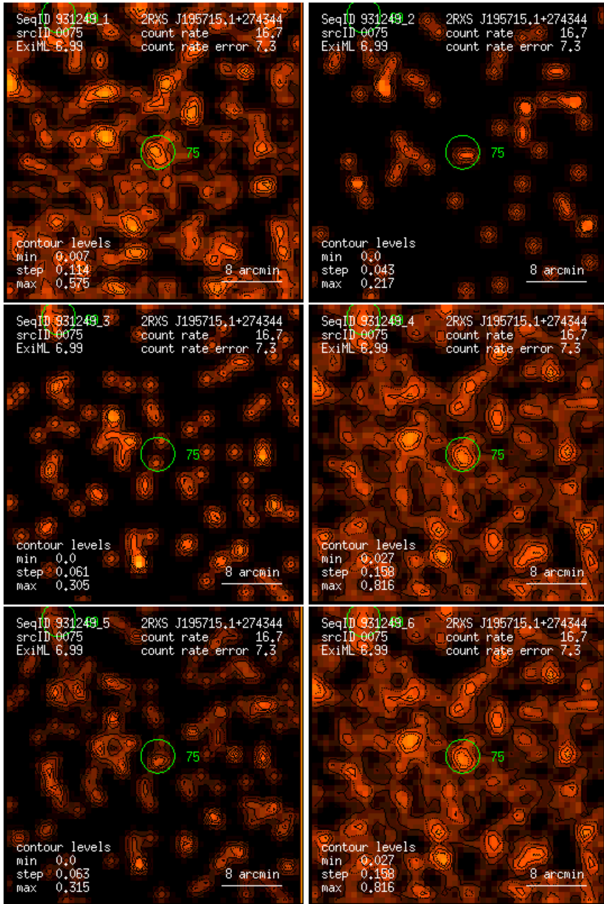
Figure 75: RASS 931249: detection 0075: band rate images, Gaussian filter: (1) PSPC channels 11 – 41, (2) 52 – 90, (3) 91 – 201, (4) 11 – 235, (5) 52 – 201, (6) 11 – 201. Broad band rates in counts/ks. Band rate contour levels in counts/ks/arcmin 2 .
