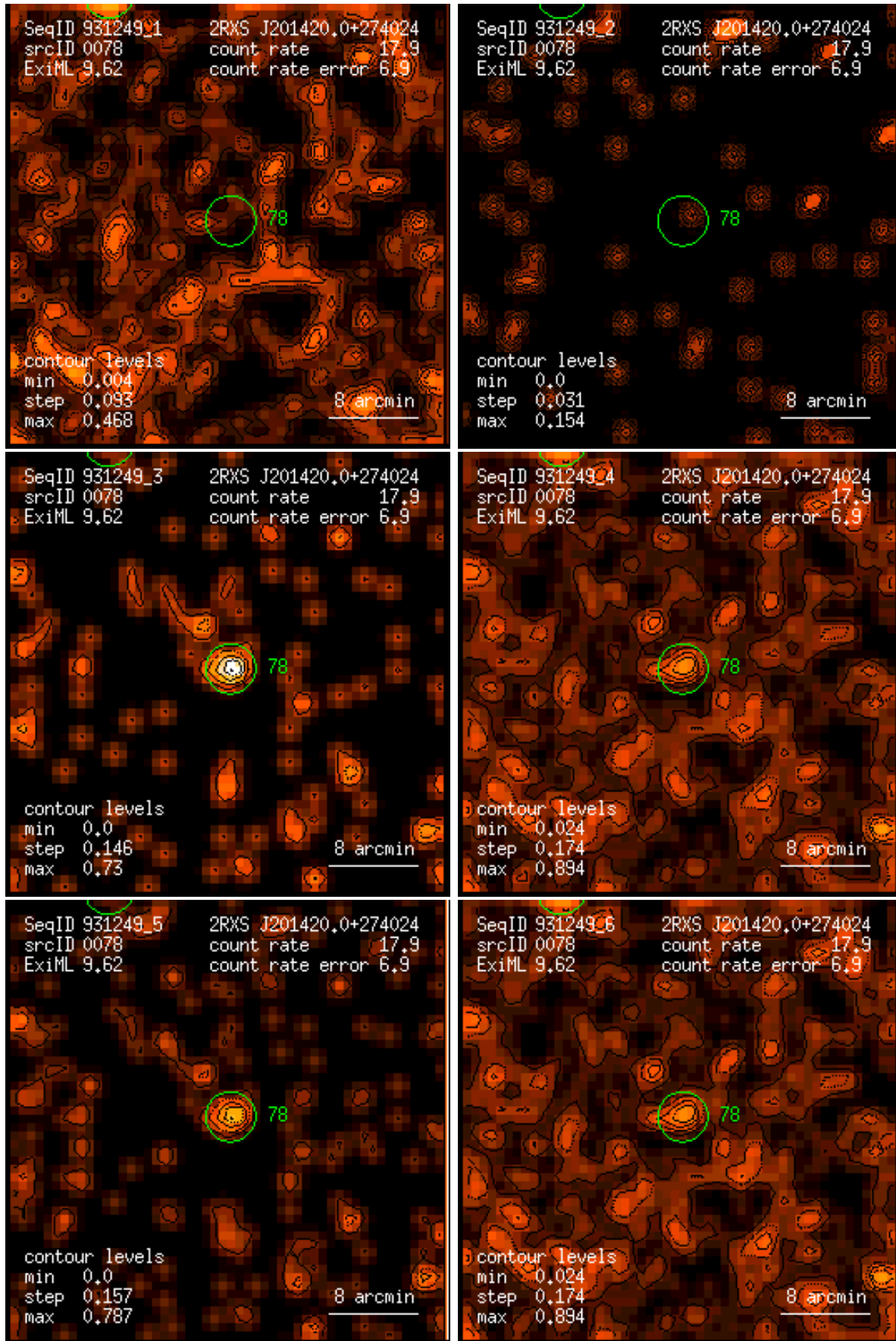
Figure 78: RASS 931249: detection 0078: band rate images, Gaussian filter: (1) PSPC channels 11 – 41, (2) 52 – 90, (3) 91 – 201, (4) 11 – 235, (5) 52 – 201, (6) 11 – 201. Broad band rates in counts/ks. Band rate contour levels in counts/ks/arcmin 2 .
