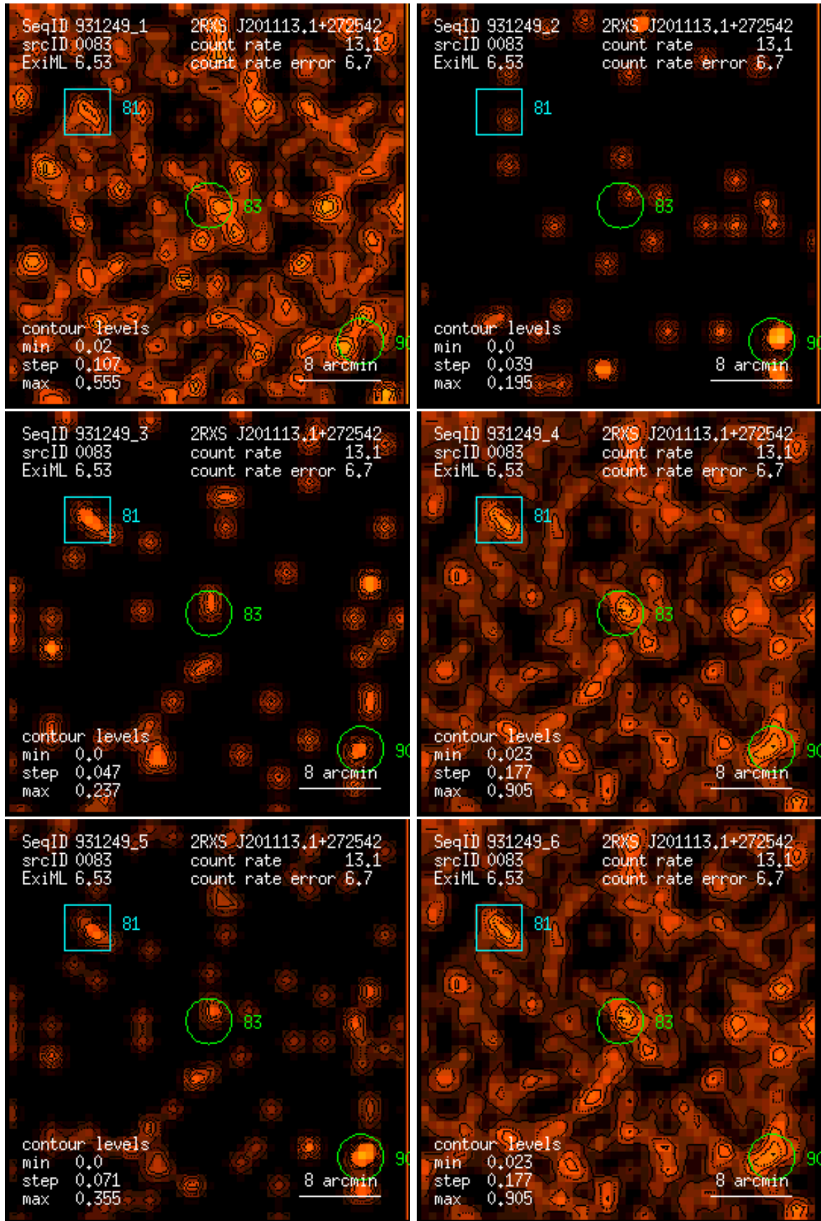
Figure 83: RASS 931249: detection 0083: band rate images, Gaussian filter: (1) PSPC channels 11 – 41, (2) 52 – 90, (3) 91 – 201, (4) 11 – 235, (5) 52 – 201, (6) 11 – 201. Broad band rates in counts/ks. Band rate contour levels in counts/ks/arcmin 2 .
