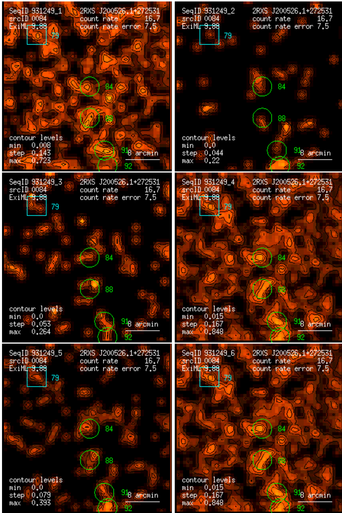
Figure 84: RASS 931249: detection 0084: band rate images, Gaussian filter: (1) PSPC channels 11 – 41, (2) 52 – 90, (3) 91 – 201, (4) 11 – 235, (5) 52 – 201, (6) 11 – 201. Broad band rates in counts/ks. Band rate contour levels in counts/ks/arcmin 2 .
