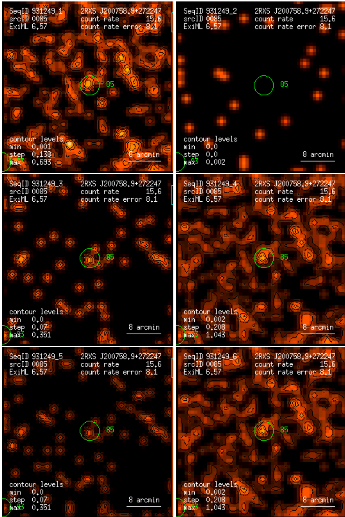
Figure 85: RASS 931249: detection 0085: band rate images, Gaussian filter: (1) PSPC channels 11 – 41, (2) 52 – 90, (3) 91 – 201, (4) 11 – 235, (5) 52 – 201, (6) 11 – 201. Broad band rates in counts/ks. Band rate contour levels in counts/ks/arcmin 2 .
