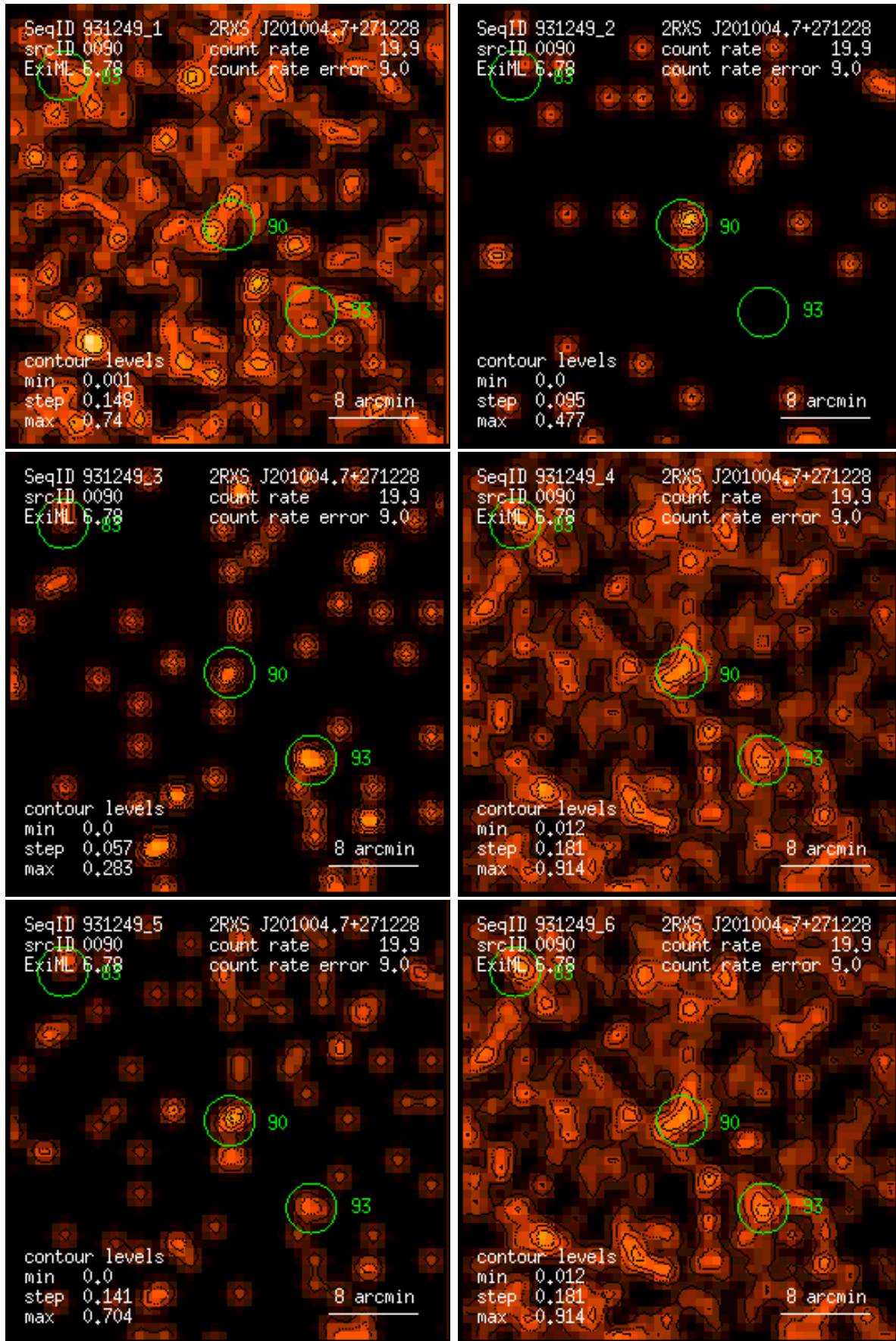
Figure 90: RASS 931249: detection 0090: band rate images, Gaussian filter: (1) PSPC channels 11 – 41, (2) 52 – 90, (3) 91 – 201, (4) 11 – 235, (5) 52 – 201, (6) 11 – 201. Broad band rates in counts/ks. Band rate contour levels in counts/ks/arcmin 2 .
