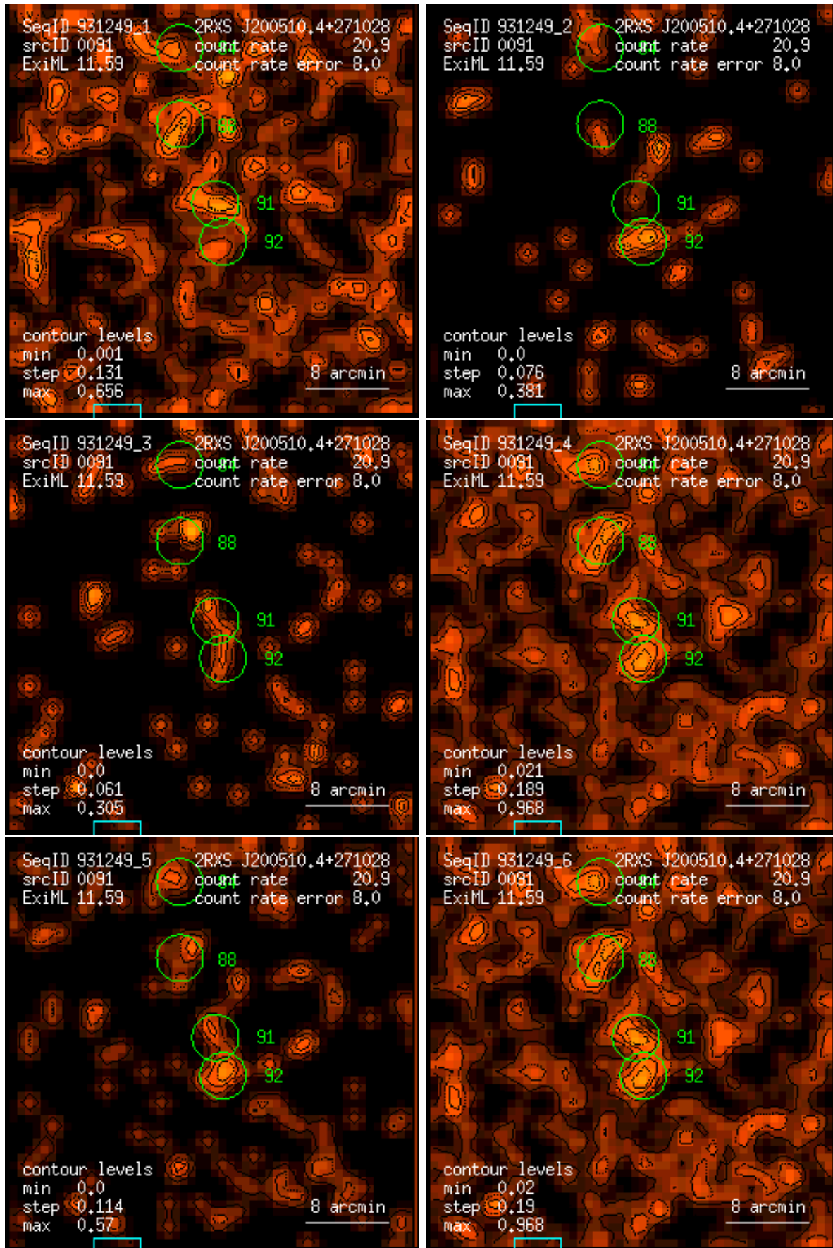
Figure 91: RASS 931249: detection 0091: band rate images, Gaussian filter: (1) PSPC channels 11 – 41, (2) 52 – 90, (3) 91 – 201, (4) 11 – 235, (5) 52 – 201, (6) 11 – 201. Broad band rates in counts/ks. Band rate contour levels in counts/ks/arcmin 2 .
